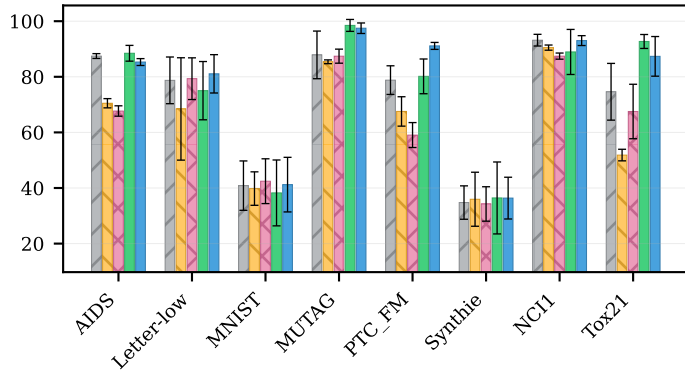
GNNExplainer
