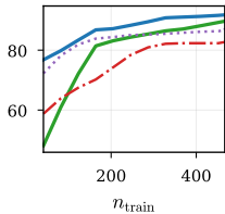
GraphSAGE
