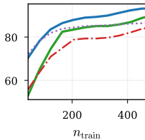
GraphSAGE
