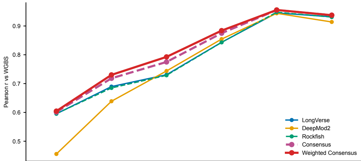
Agreement by read depth, chromosome 22
