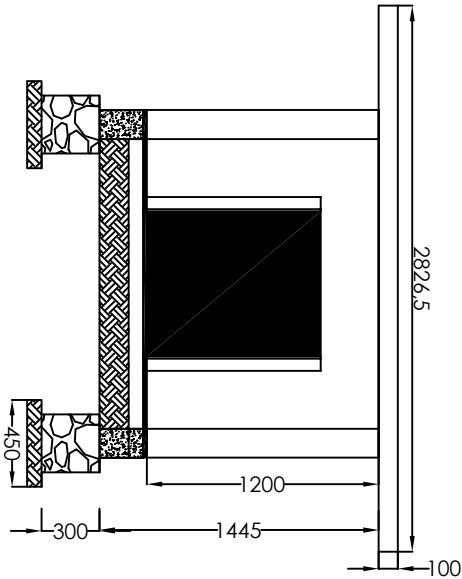
SEC.ELEVATION
