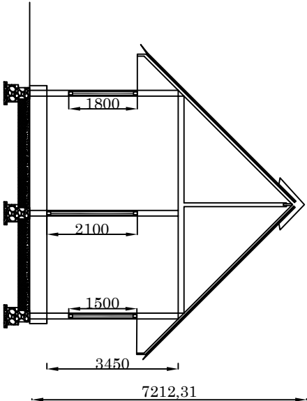
SECTION ELEVATION
