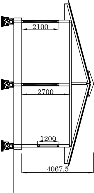
SECTION ELEVATION
