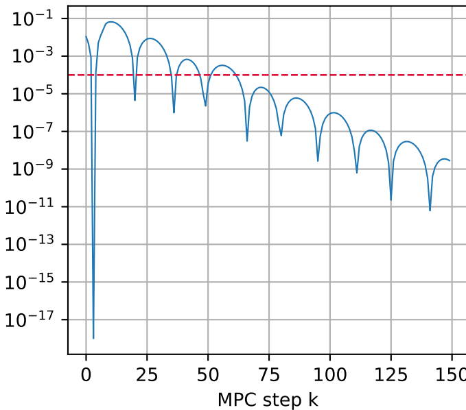
pendcart (65% benign)
