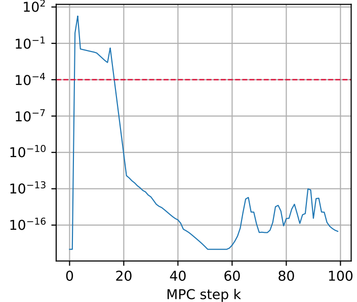
cstr (85% benign)
