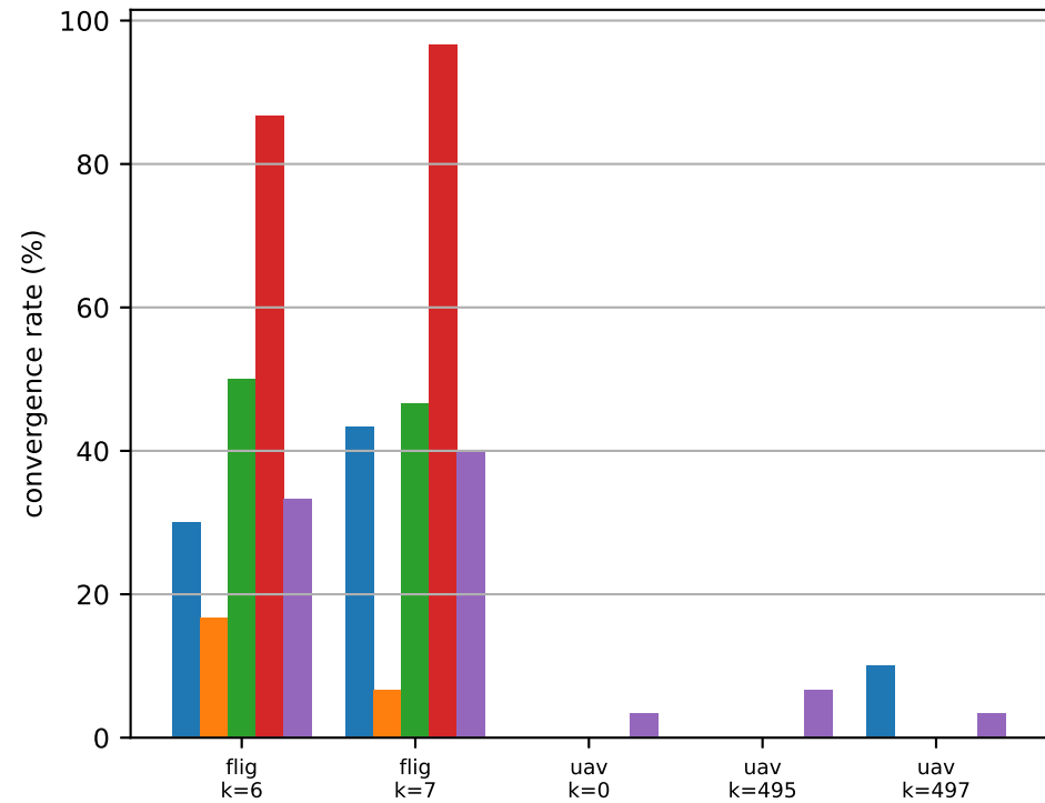
(c) plateau instances, 5000 FE
