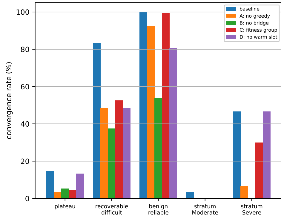
(a) 1000 FE, by instance role
