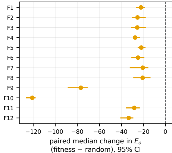
(b) filled: Holm-significant
