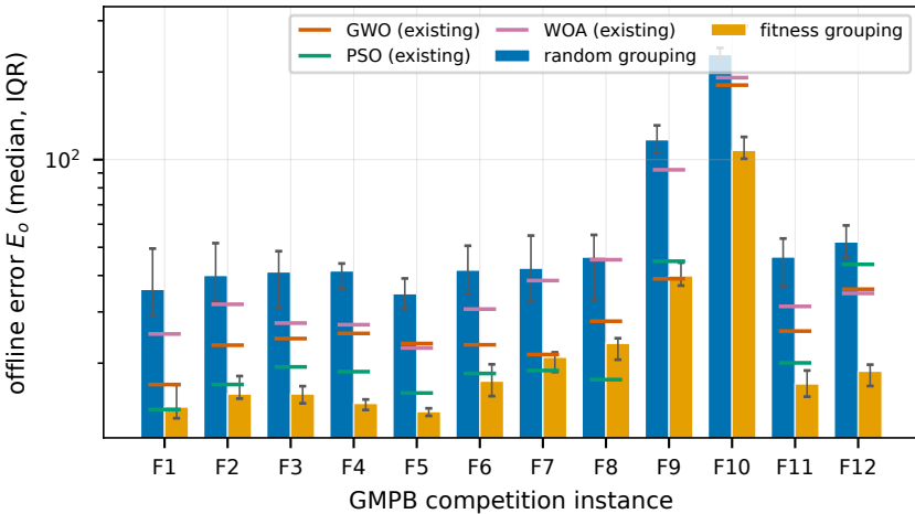
(a) SGO under two grouping rules; controls shown for context only
