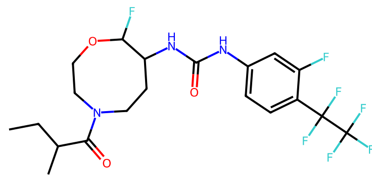
generated_002 Parent Tanimoto = 0.51
