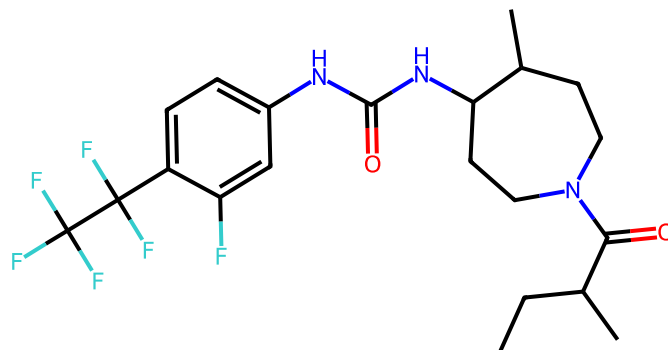
generated_001 Parent Tanimoto = 0.55
