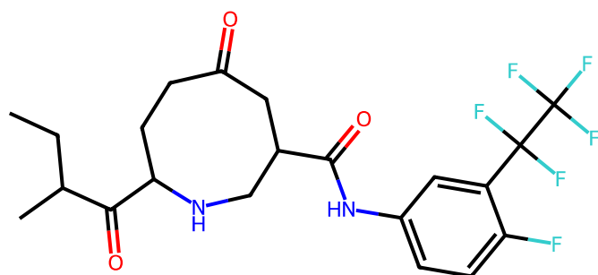
generated_003 Parent Tanimoto = 0.30
