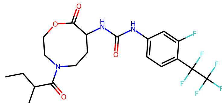
generated_005 Parent Tanimoto = 0.51
