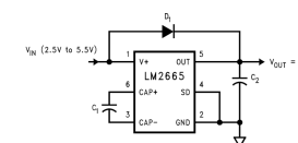
Figure 11. Voltage Doubler
