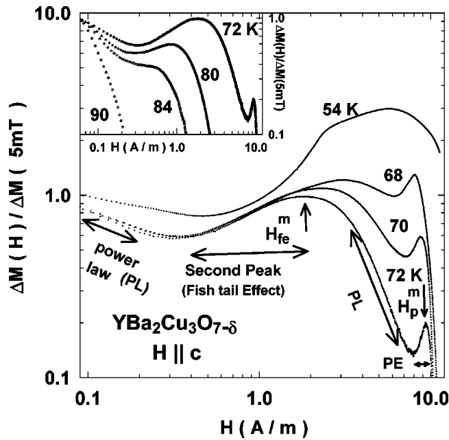
FIG. 3. Plot of the normalized J_c [\alpha \Delta M(H) / \Delta M(5 \text{ mT})] versus H at various temperatures. The demarcation of the entire field scan at 72 K into different regions, such as power law, second peak (or FE), PE, etc., is shown along with the positions of the maxima of FE and PE. The inset shows the normalized plots at T \geq 72 \text{ K} .
