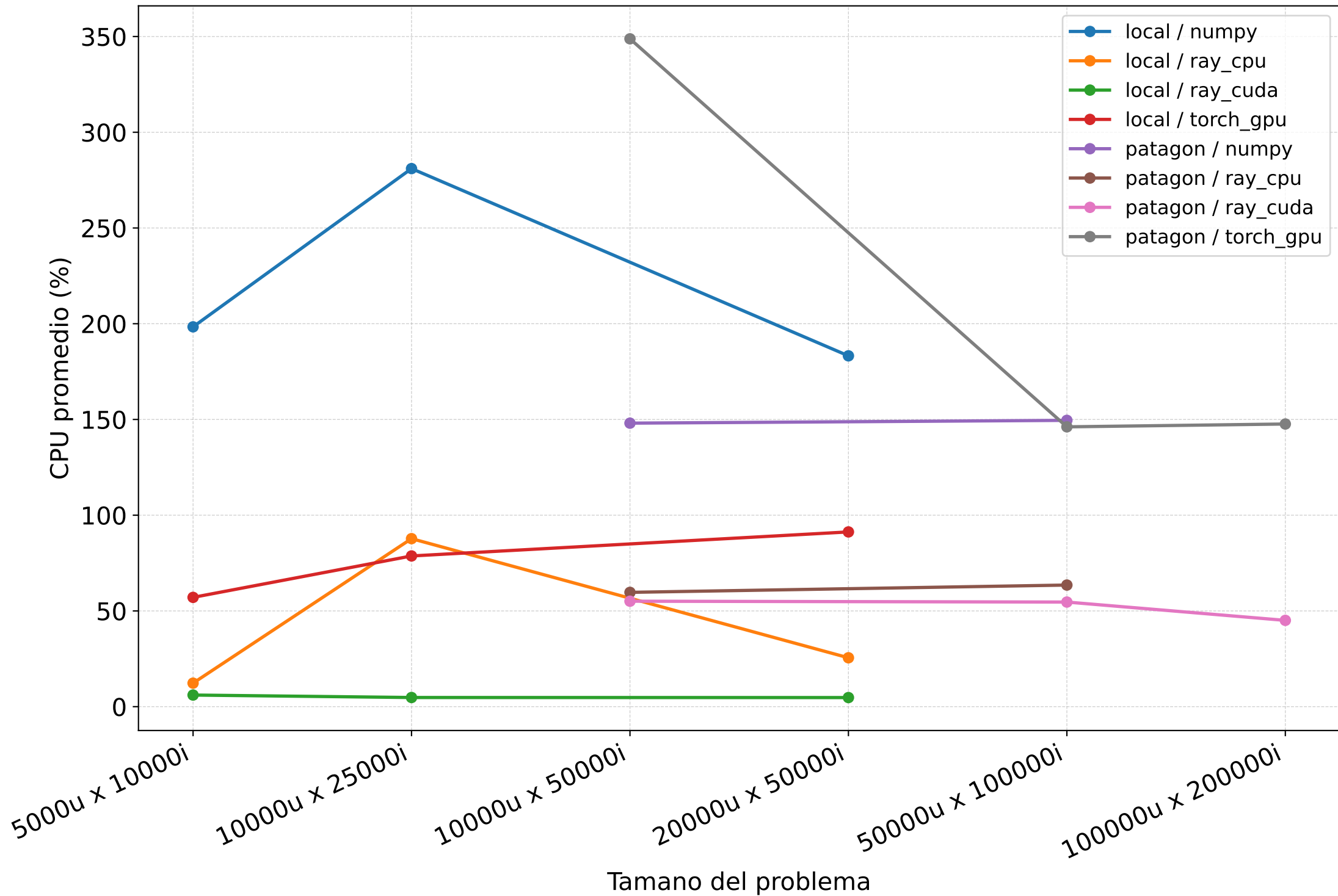
Benchmark recomendador content-based: CPU promedio (%)
