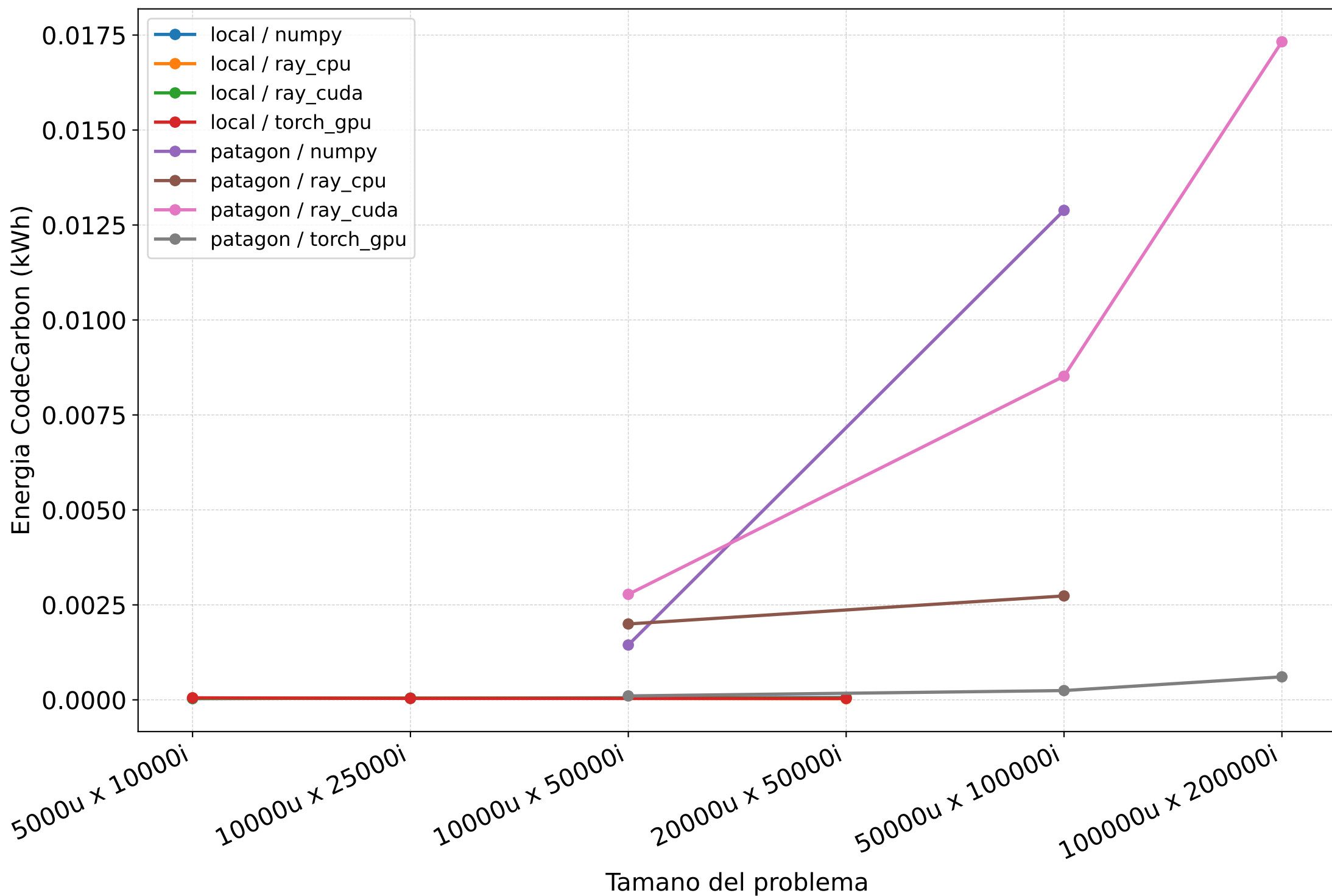
Benchmark recomendador content-based: Energia CodeCarbon (kWh)
