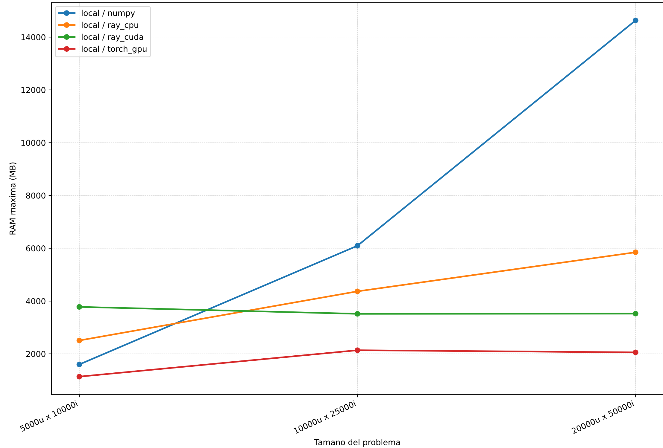
Benchmark recomendador content-based: RAM maxima (MB)
