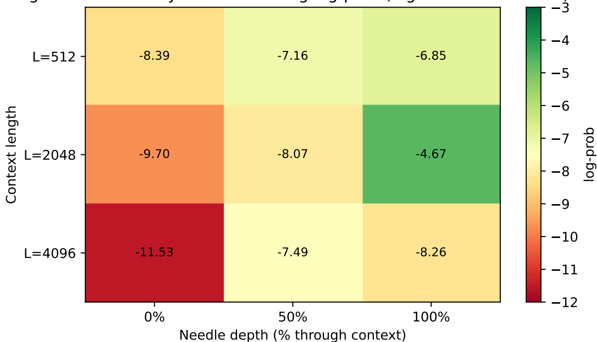
Fig 4. Needle-in-Haystack 130M: avg log-prob (higher = better recall)
