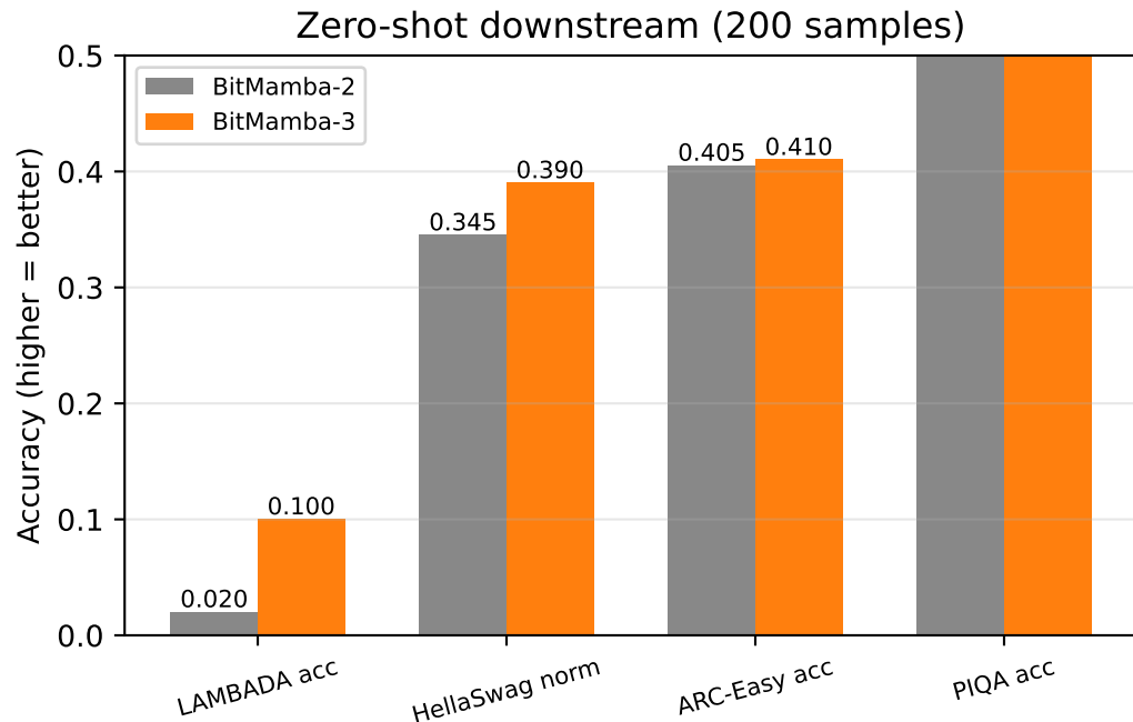
Fig 7. BitMamba-2 vs BitMamba-3 at 130M (same 480M tokens, same training)
