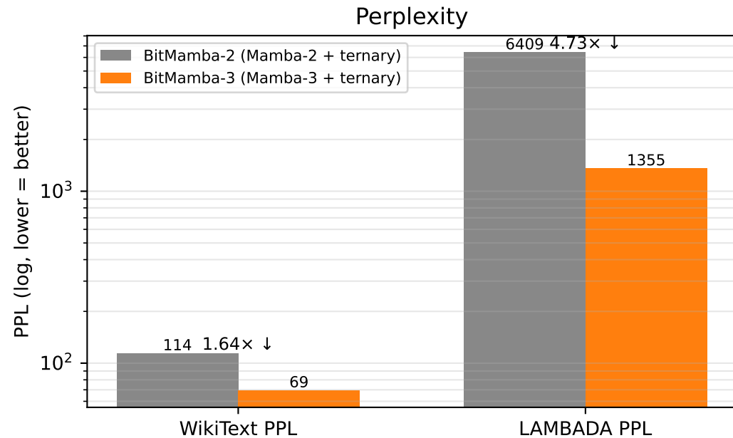
Fig 7. BitMamba-2 vs BitMamba-3 at 130M (same 480M tokens, same training)
