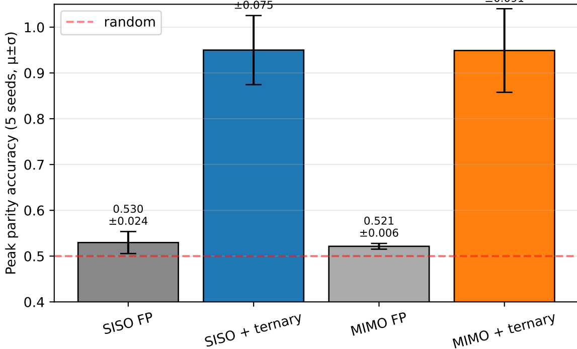
Fig 2. Ternary quantization as state-tracking inductive bias ( d=256 , \text{depth}=2 , cosine LR, 5K steps)
