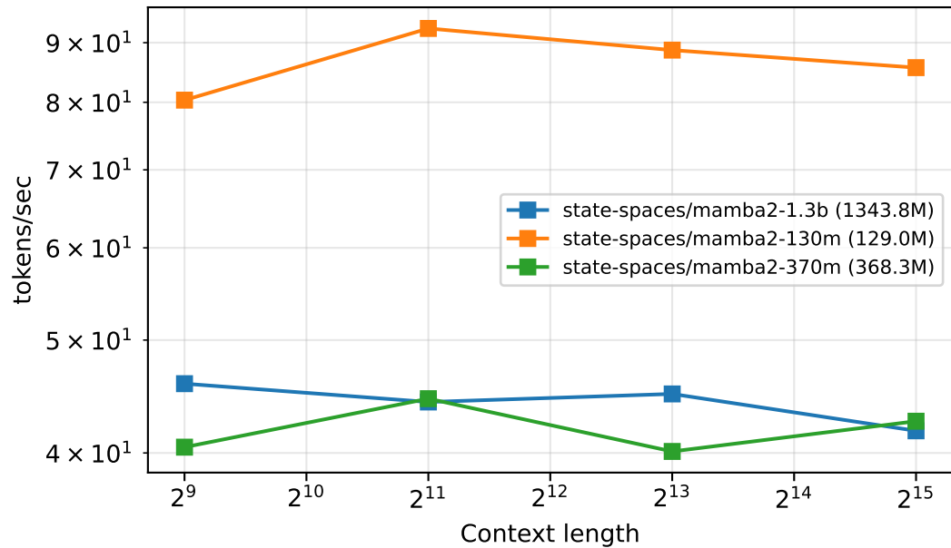
Mamba-2 FP16 Decode throughput (RTX 5090)
