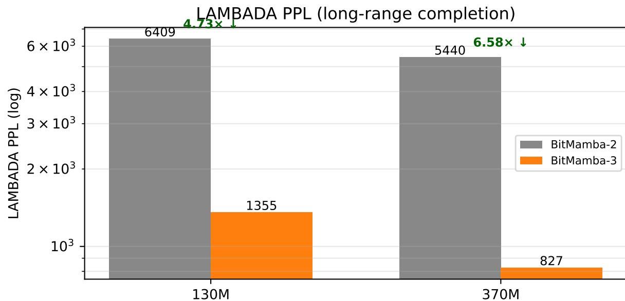
Fig 7. BitMamba-2 vs BitMamba-3 at 130M and 370M (matched 480M fineweb-edu tokens, matched ternary quantization)
