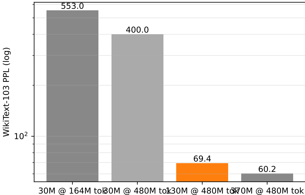
Fig 3. BitMamba-3 PPL scaling: model size + training tokens
