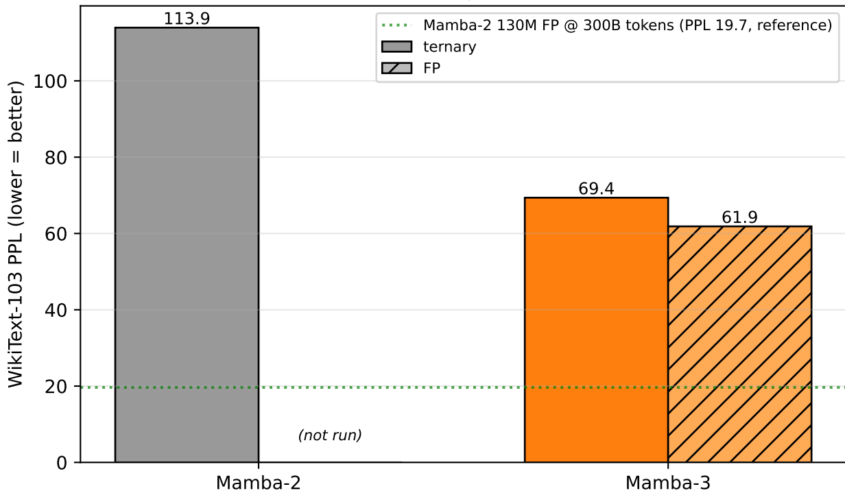
Fig 8. Architecture \times Quantization decomposition at 130M / 480M tokens M2 \rightarrow M3 (ternary): 1.64 \times advantage | FP \rightarrow ternary (M3): +12.1% PPL cost
