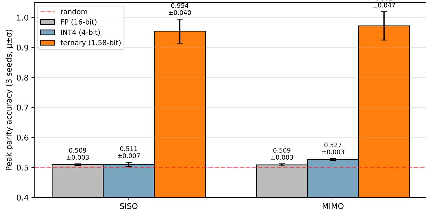
Fig 9. Inductive bias is specific to ternary, not generic low-bit (d=512, depth=4, cosine LR, 5K steps; INT4 PTQ identical to FP at chance)
