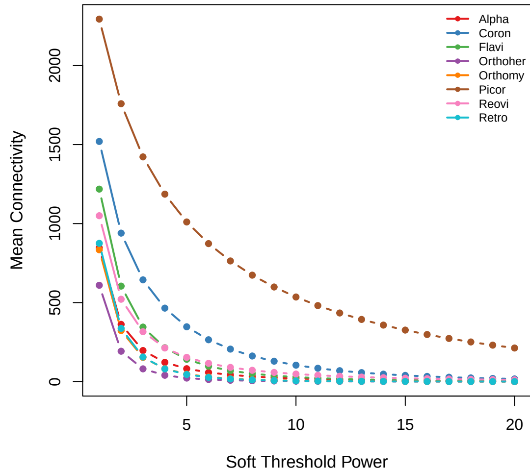
Mean Connectivity
