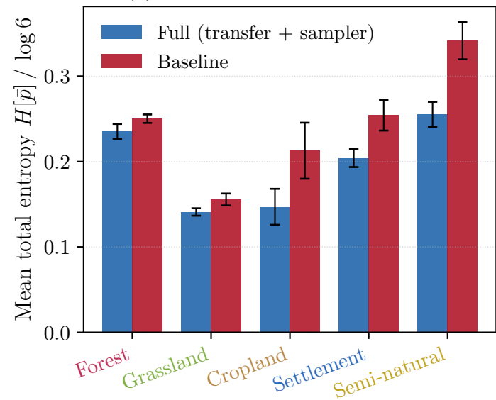
(a) Total uncertainty by GT class
