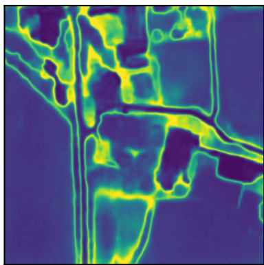
Aleatoric-type \mathbb{E}_i[H]
