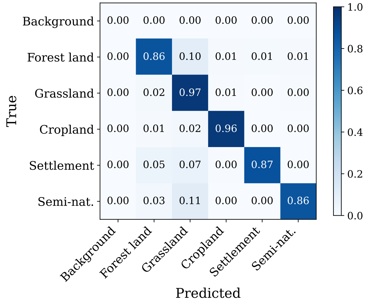
(c) Stage 5: +Knowledge Distillation
