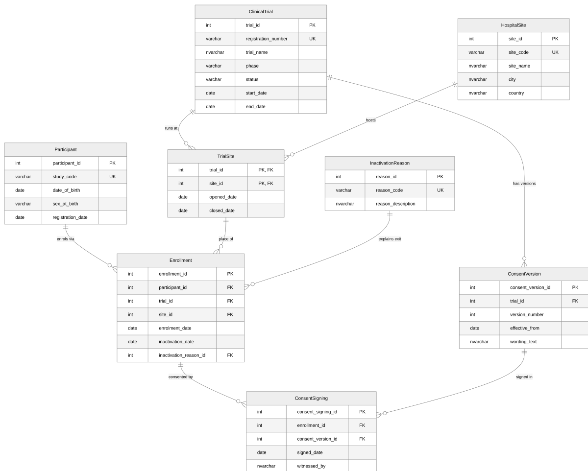
Figure 1.1: Entity Relationship Diagram (crow's-foot notation).
