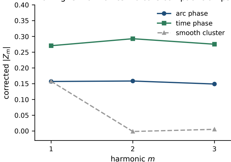
Flat higher harmonics indicate compact clumps
