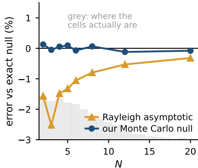
(b) The asymptotic null is biased where the data live
