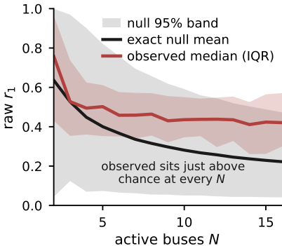
(a) Raw r_1 tracks fleet size, not coordination
