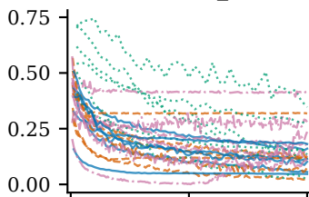
stiffness/cos_within
