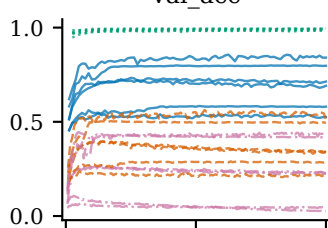
noise_scale/simple
