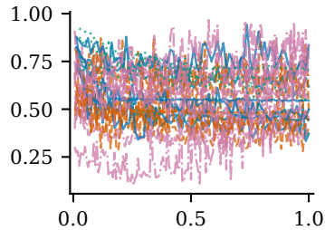
confusion/eta
