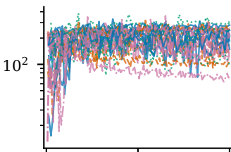
stiffness/cos_within
