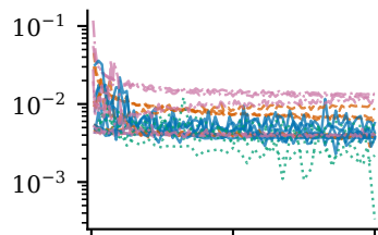
gd/scalar
