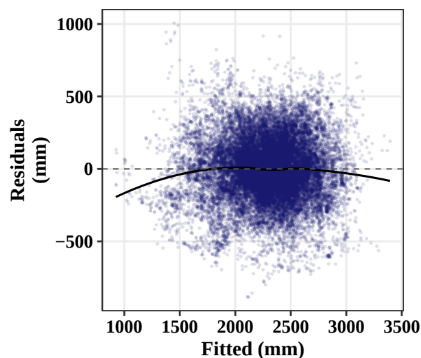
Precipitation
