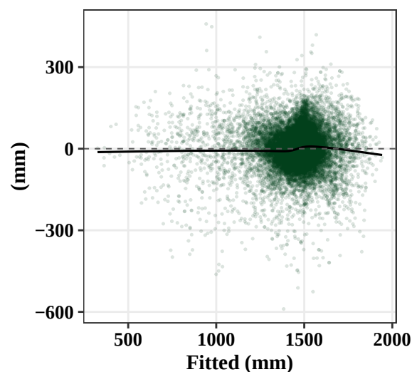
Evapotranspiration
