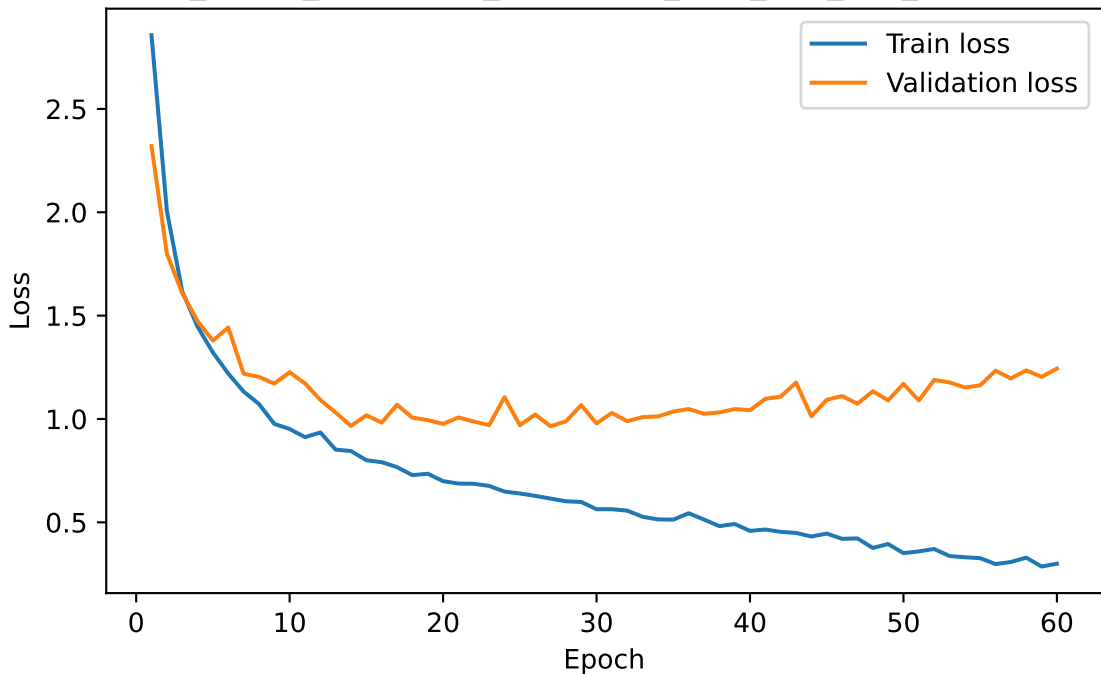
V3.8.1_fusion_taskaware_merged34_GRU_E60_L64_sorted - Loss
