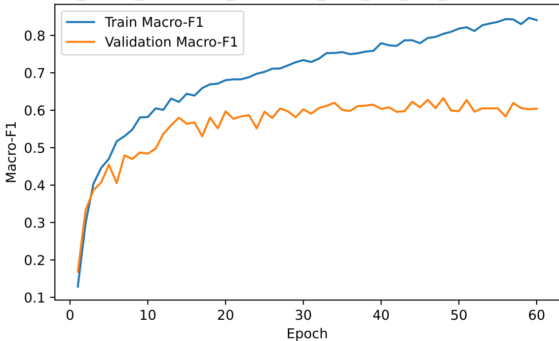
V3.8.1_fusion_taskaware_merged34_GRU_E60_L64_sorted - Macro-F1
