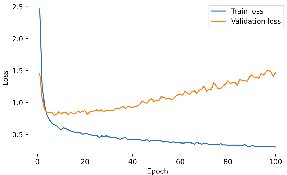
V3.8.10d_IPM_soft_history_MLP_K4_E100_dropout03_seed42 - Loss
