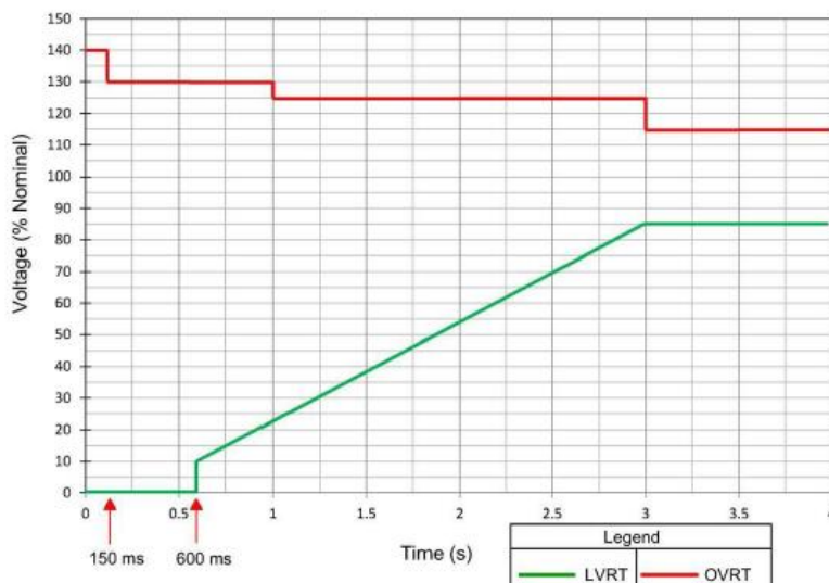
Figure 1 BESS Voltage Operational Range and Ride-Through Requirements
