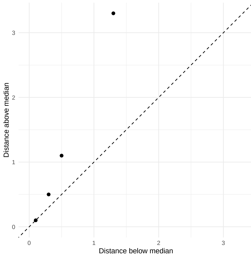
Figure 6. Symmetry plot of the paired differences from the sleep dataset, pairing each observation's distance above the median with the corresponding distance below. Under symmetry, points fall along the 45-degree reference line (dashed); systematic departures — points consistently above or below the line — indicate asymmetry. The signed-rank variant of WMW requires this symmetry for the pseudo-median to coincide with the mean or median of the differences.
