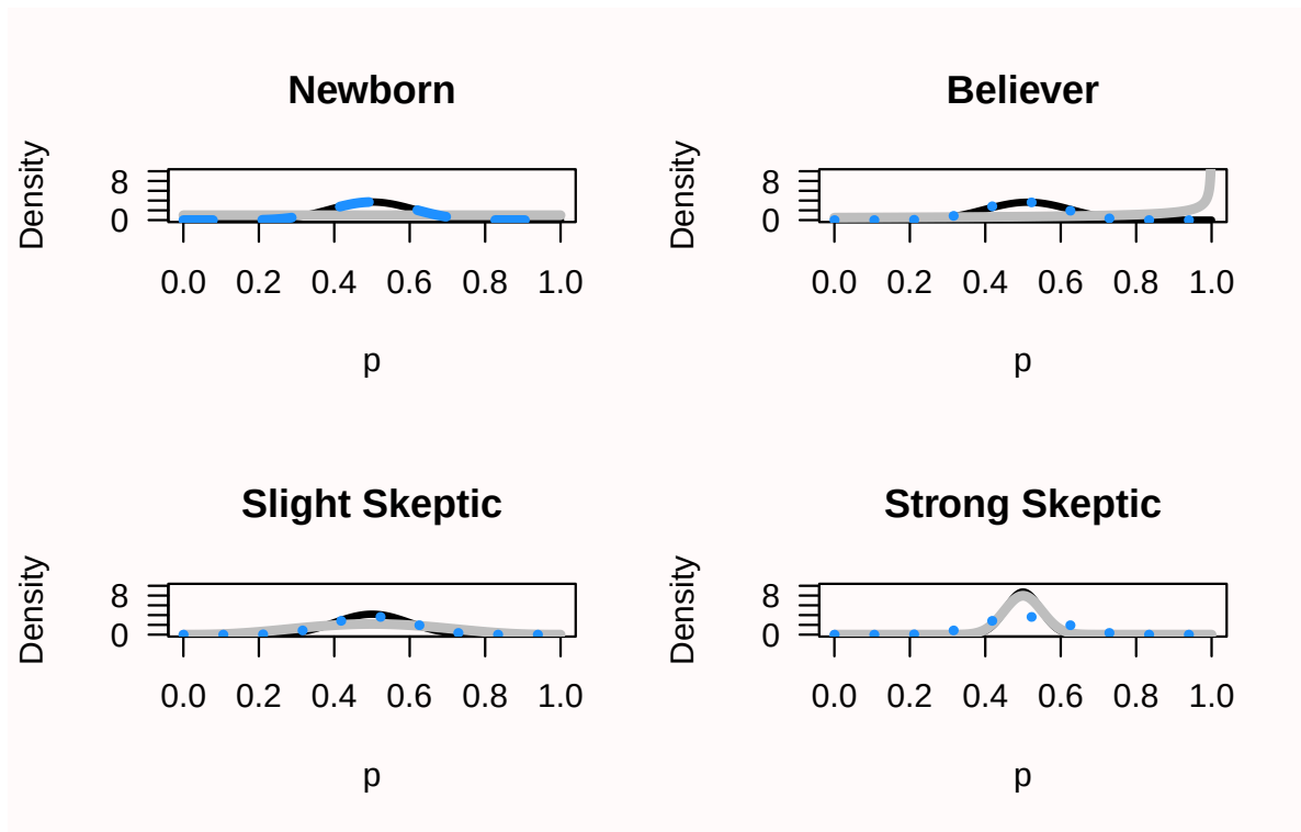
Figure 4.2: Four examples of how different priors are updated to the posterior based on data.
