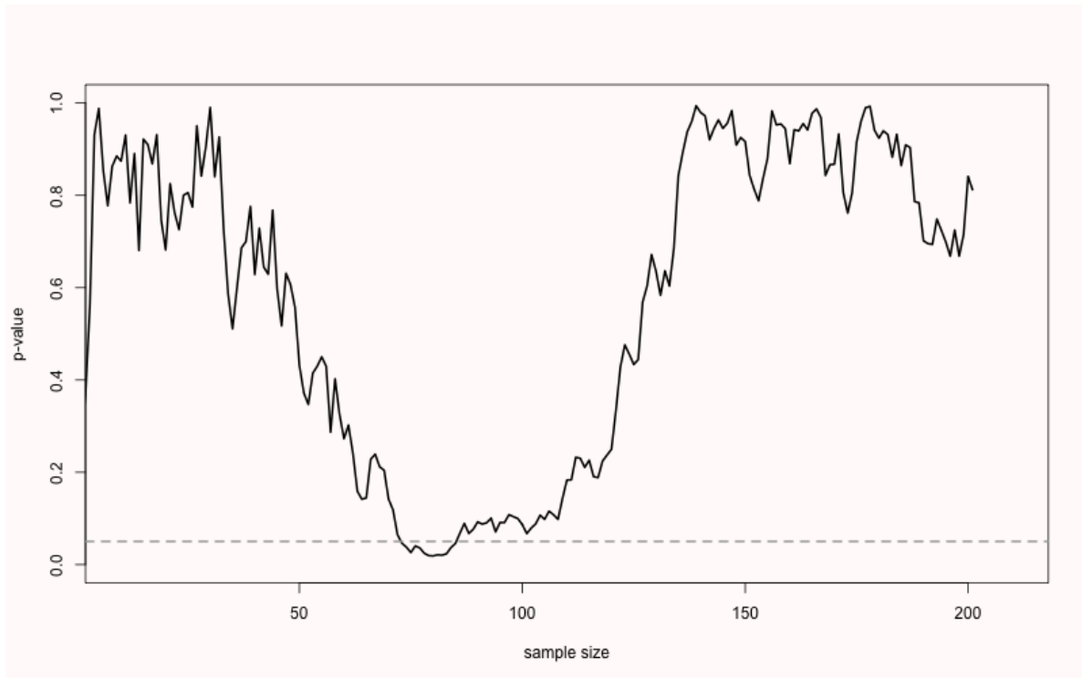
Figure 2.6: Simulated p -values for each additional observation when the null is true.
