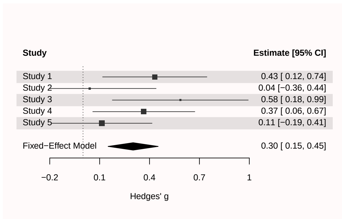
Figure 11.9: Simulated studies under a fixed effect model.
