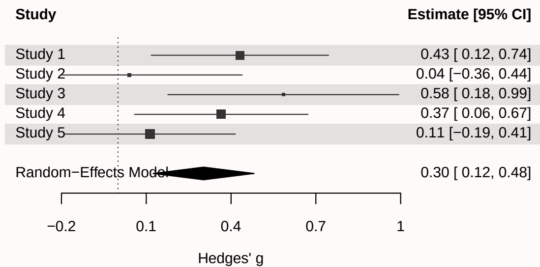
Figure 11.8: Simulated studies under a random effects model.
