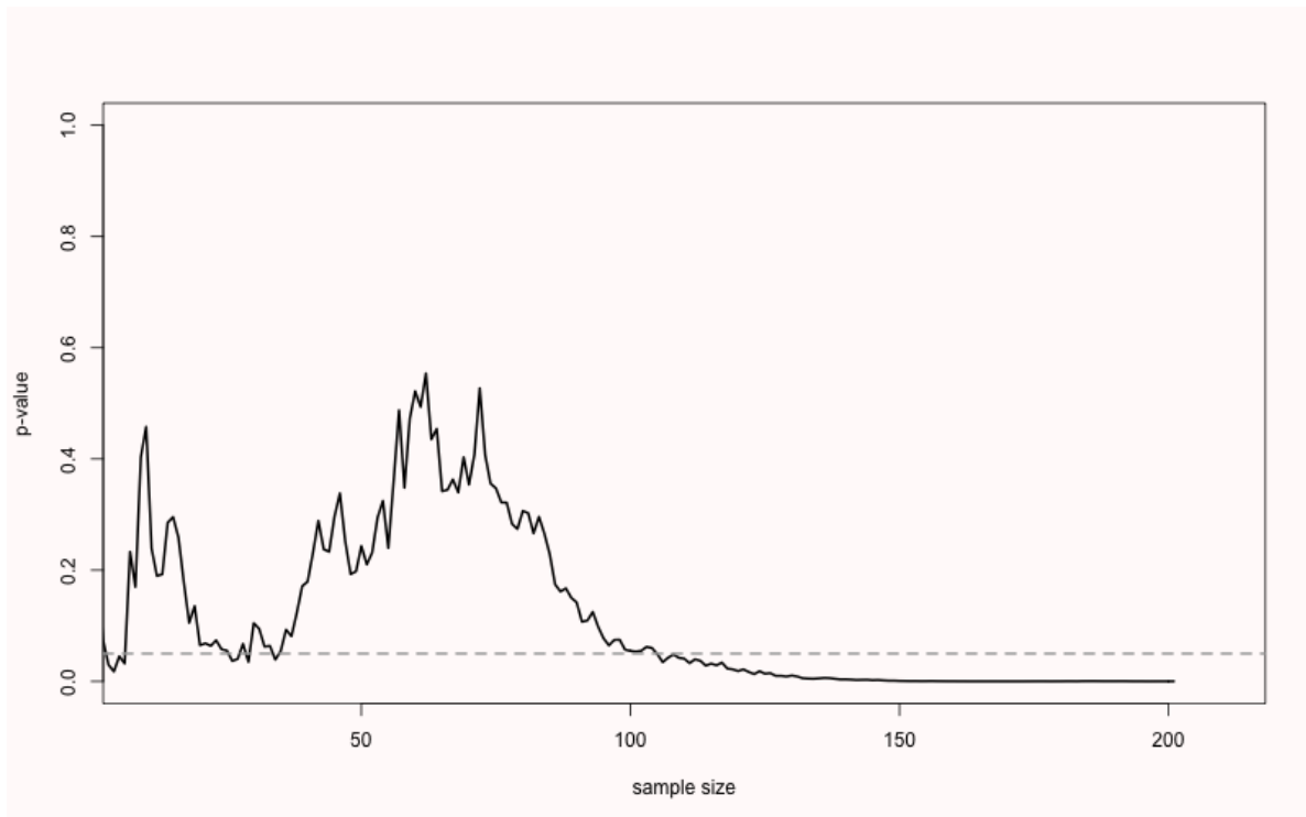
Figure 2.7: Simulated p -values for each additional observation when d = 0.3 .
