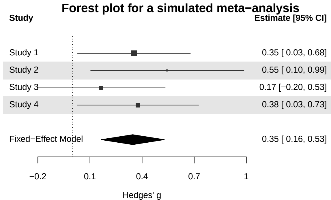
Figure 7.9: Meta-analysis of 4 studies.
