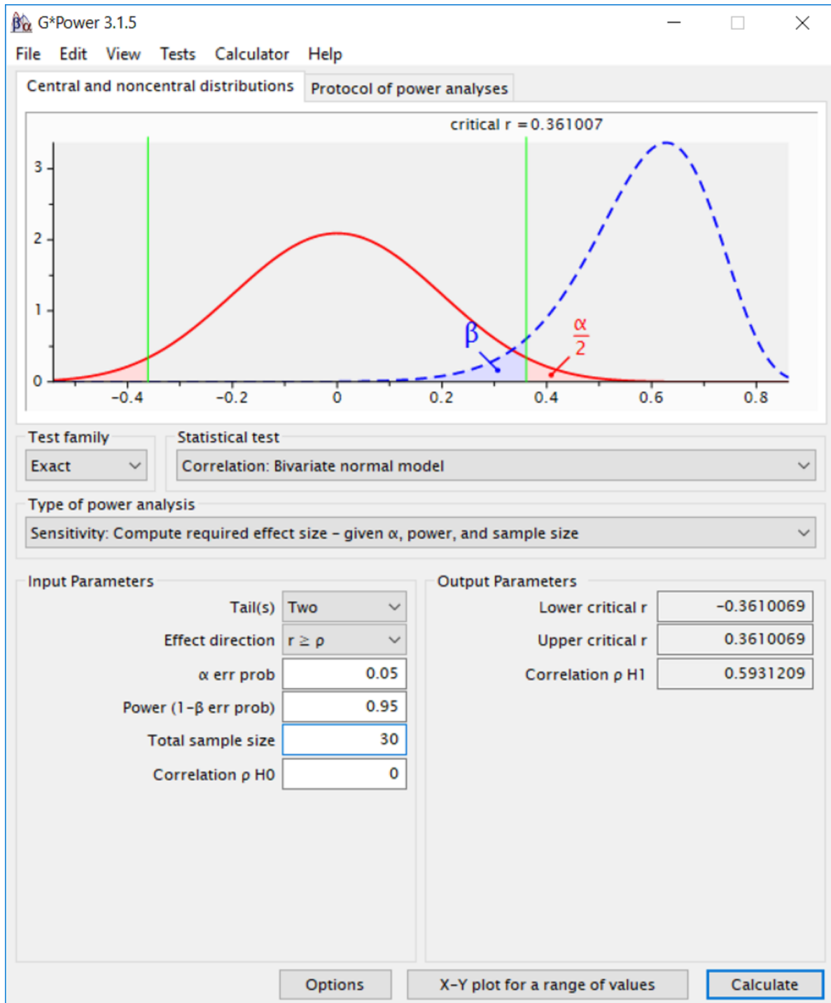
Figure 6.10: The critical correlation of a test based on a total sample size of 30 and \alpha = 0.05 calculated in G*Power.
