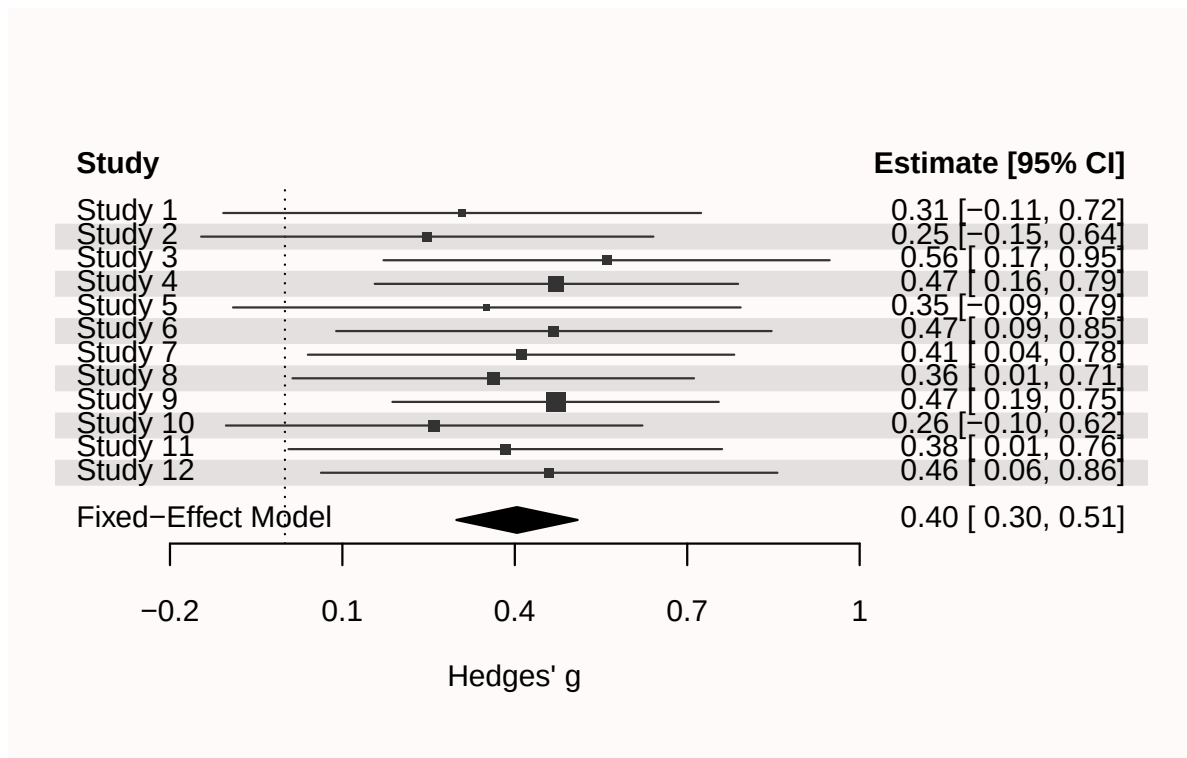
Figure 11.5: Forest plot for 12 simulated studies.
