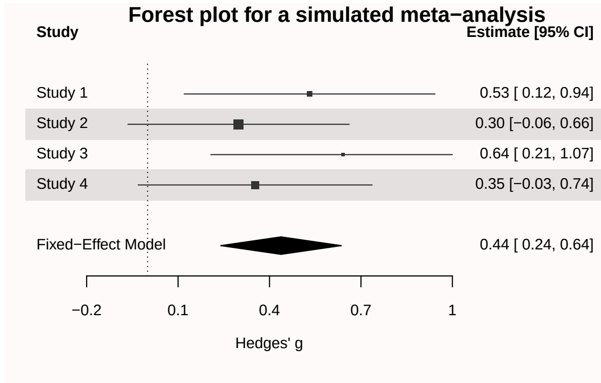
Figure 7.3: Meta-analysis of 4 studies.
