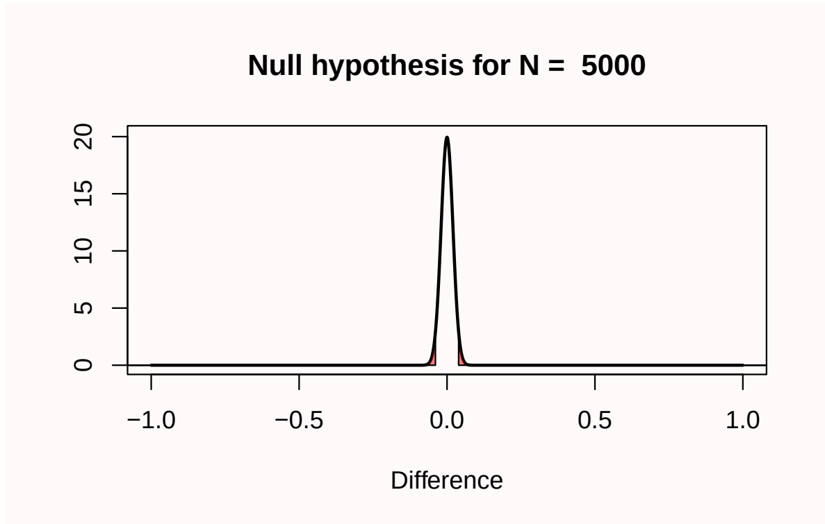
Figure 1.4: Distribution of observed Cohen's d effect sizes when collecting 5000 observations per group in an independent t -test when d = 0 .
