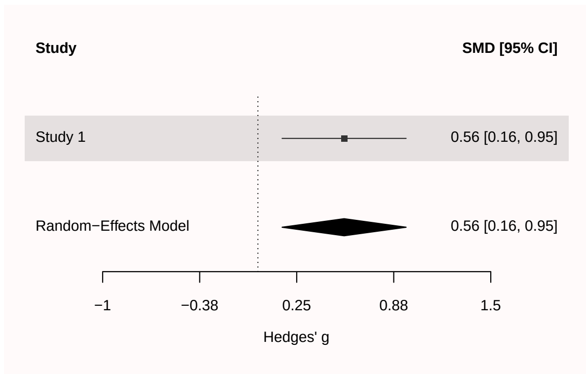
Figure 11.4: Forest plot for a single study.
