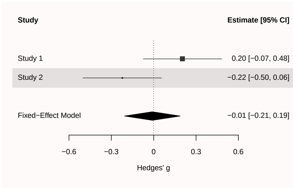
Figure 7.5: Meta-analysis of two simulated studies from the same population.
