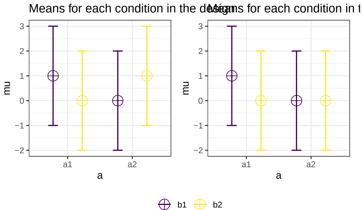
Figure 6.8: Disordinal (or cross-over) and ordinal interaction with means of 0 and 1, n = 50 per group, and an SD of 2.
