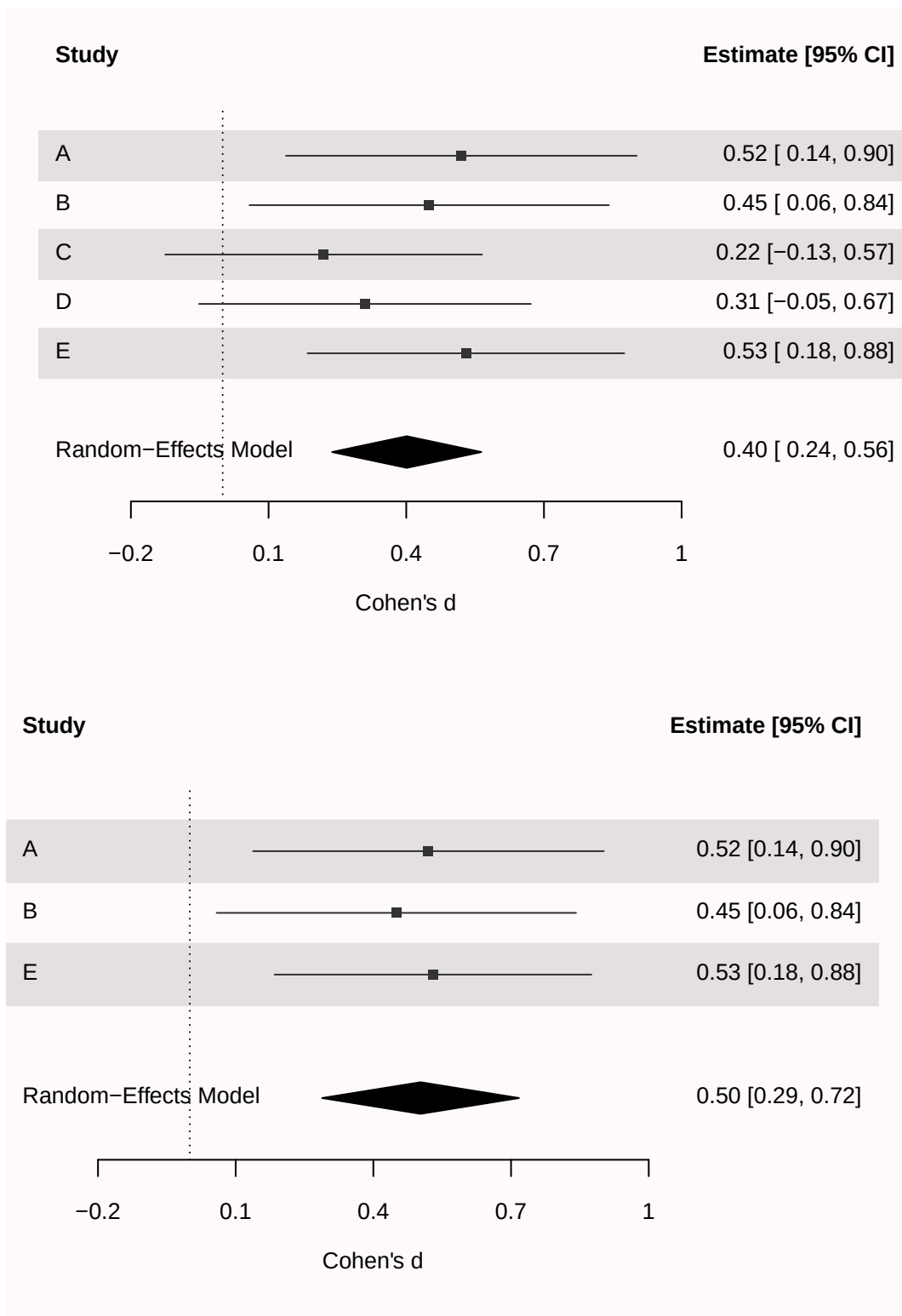
Figure 6.9: Two forest plots, the top with all studies reported, the bottom only reporting statistically significant effects.
