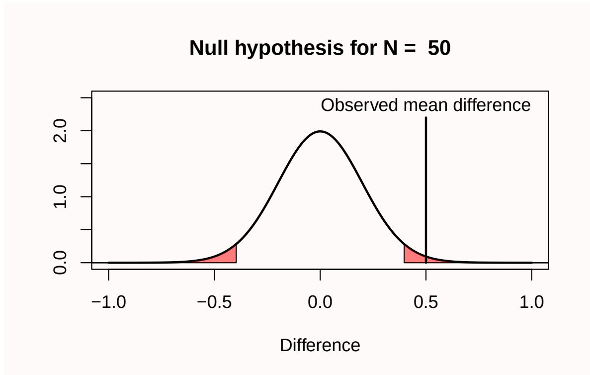
Figure 1.8: Distribution of observed Cohen's d effect sizes when collecting 50 observations per group in an independent t -test when d = 0 and observing d = 0.5 .
