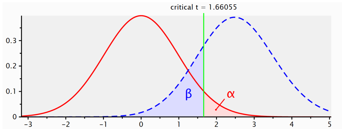
Figure 1.5: Screenshot from G*Power software visualizing the distributions of t -values of the null model (in red) and the alternative model (in blue) and the critical t -value (1.66055), i.e. the threshold distinguishing significant from non-significant results.
