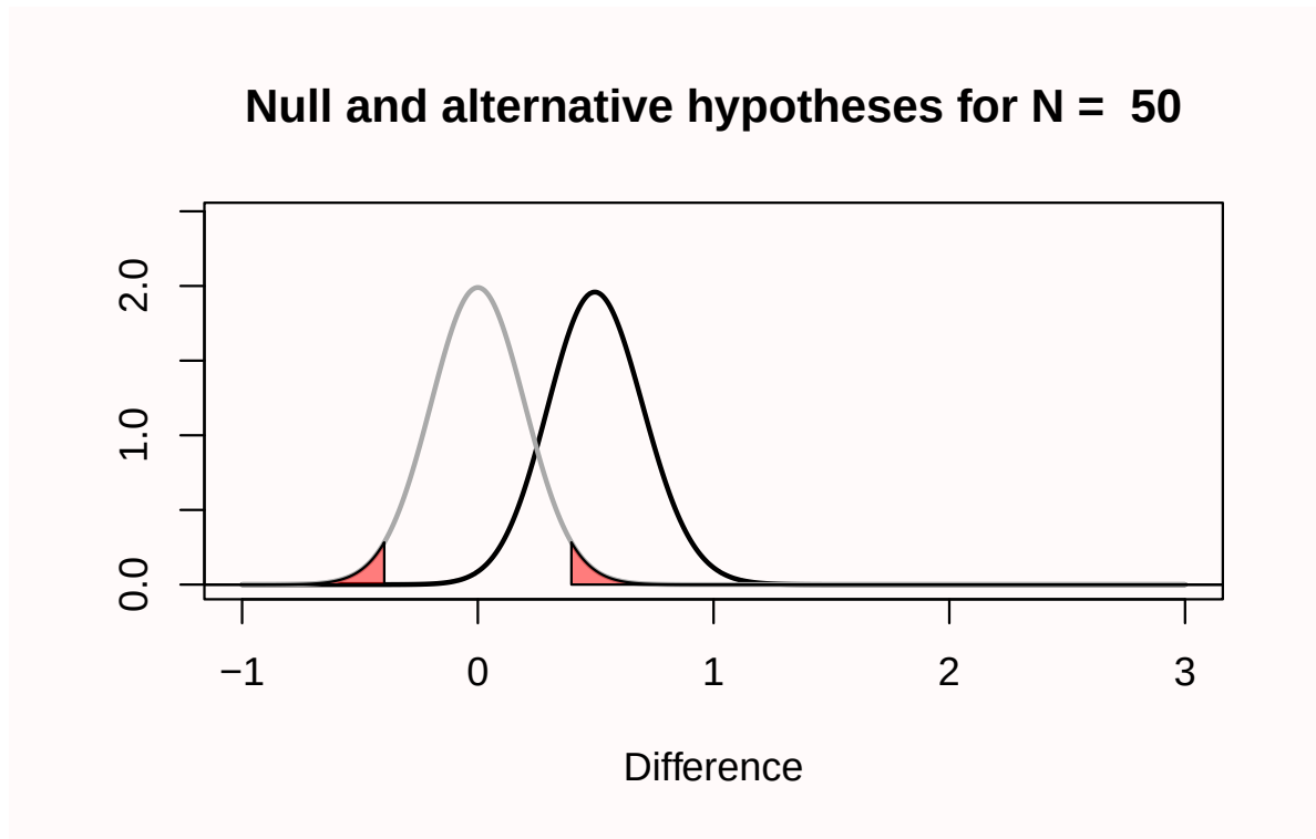
Figure 1.6: Distribution of observed Cohen's d effect sizes when collecting 50 observations per group in an independent t -test when d = 0 (null model, left) or d = 0.5 (alternative model, right).
