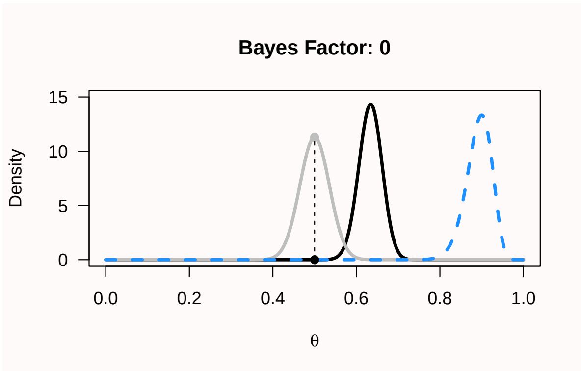
Figure 4.1: Plot for a strongly informed prior, the likelihood, and the posterior.
