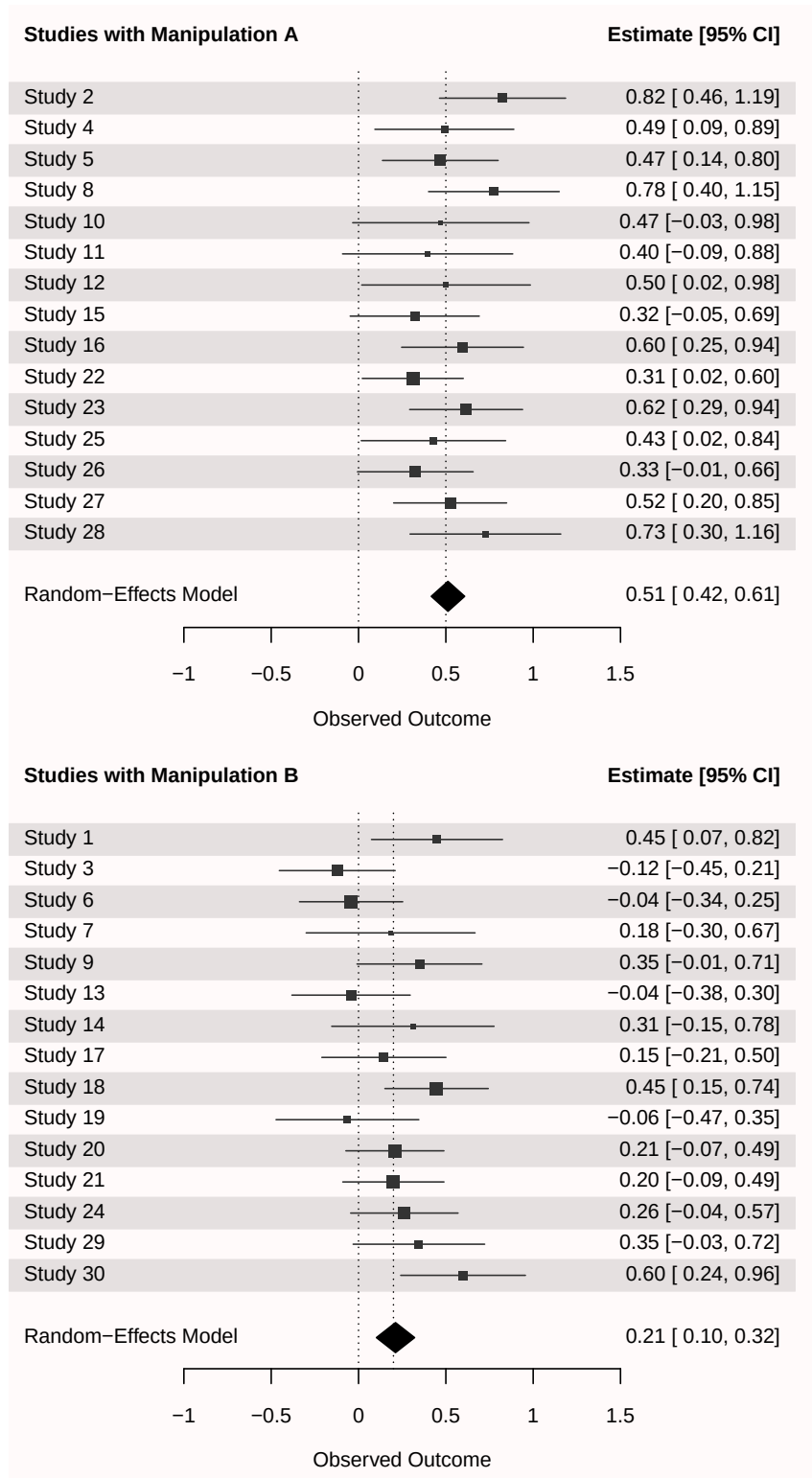
Figure 11.7: Two forest plots for the 2 different subgroups with Manipulation A or B.
