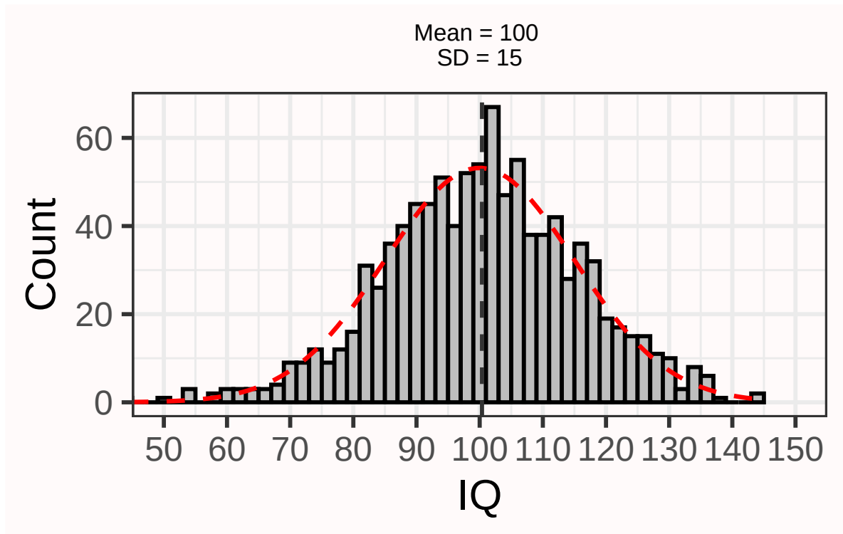
Figure 11.1: 1000 random datapoints with mean = 100 and sd = 15 in the population.
