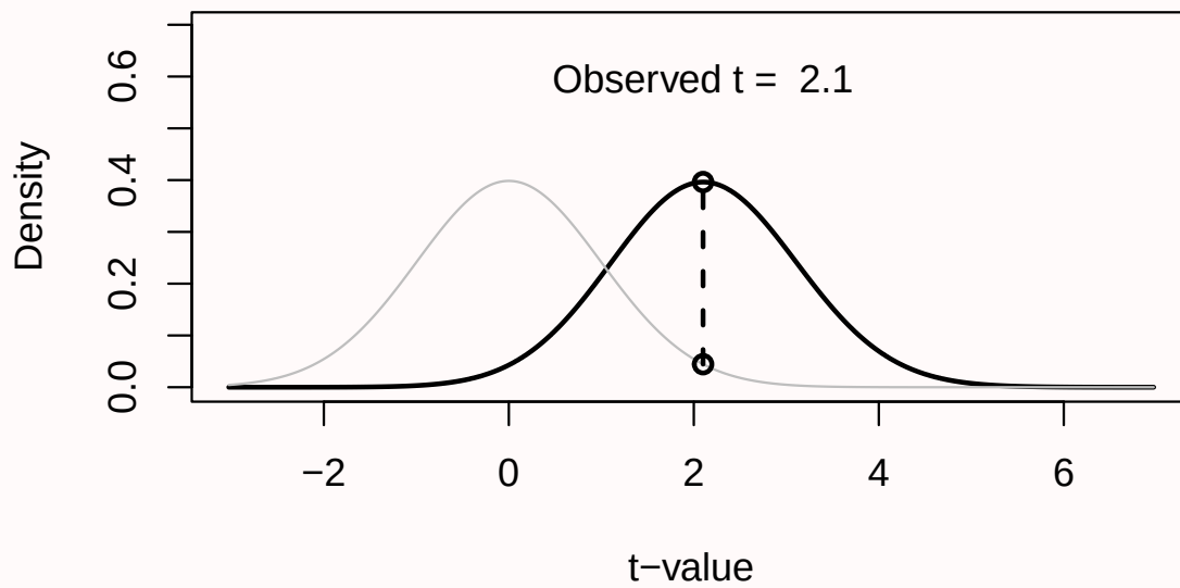
Figure 3.8: Likelihood ratio for observed t -value under H_0 and H_1 .
