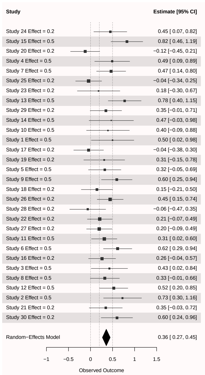
Figure 11.6: Forest plot of 30 studies with 2 subsets of studies, one set with a true effect size of 0.2, and one set with a true effect size of 0.5.
