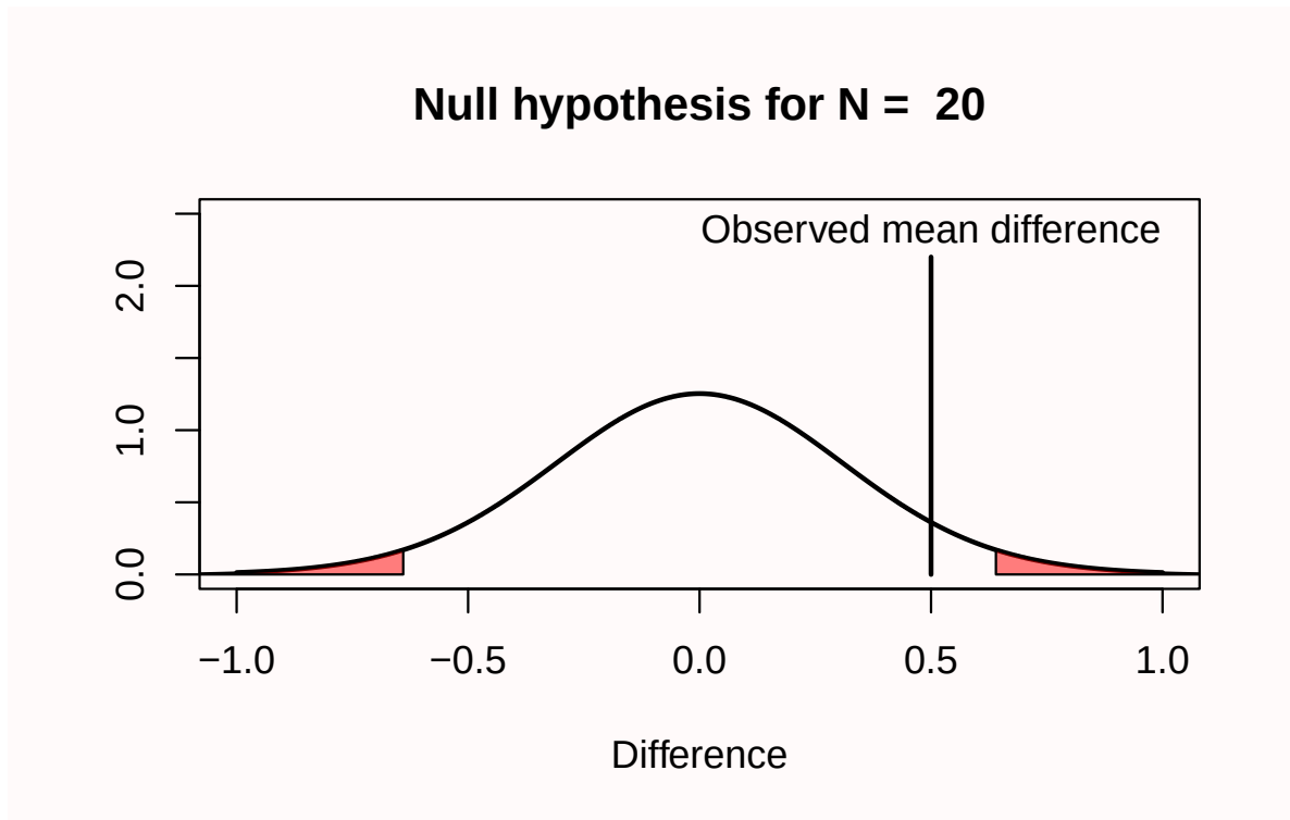
Figure 1.9: Distribution of observed Cohen's d effect sizes when collecting 20 observations per group in an independent t -test when d = 0 .
