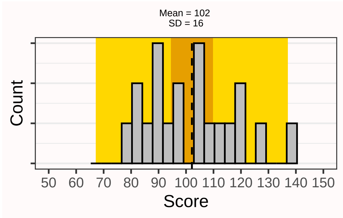
Figure 7.4: A comparison of a 95% confidence interval (orange) and 95% prediction interval (yellow).
