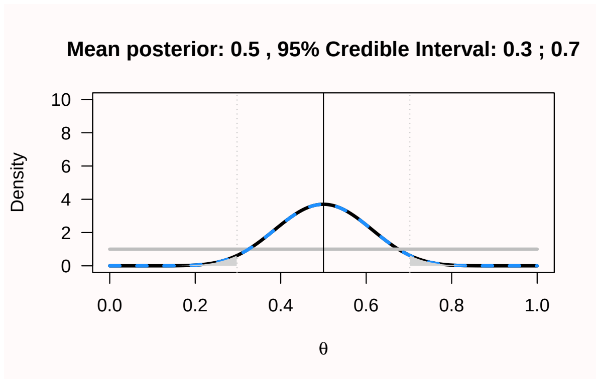
Figure 4.2: Plot for the mean of the posterior when 10 out of 20 heads are observed given a uniform prior.
