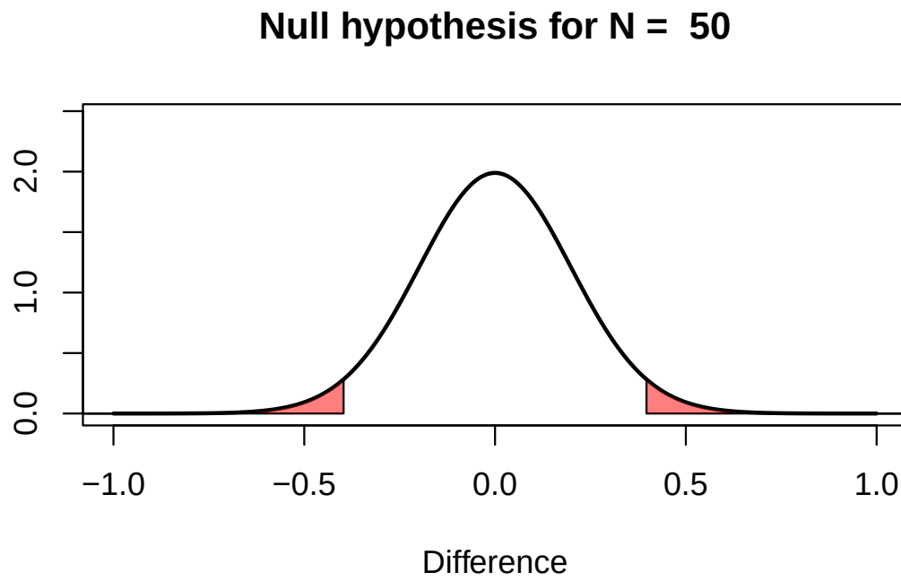
Figure 1.3: Distribution of observed Cohen's d effect sizes when collecting 50 observations per group in an independent t -test.
