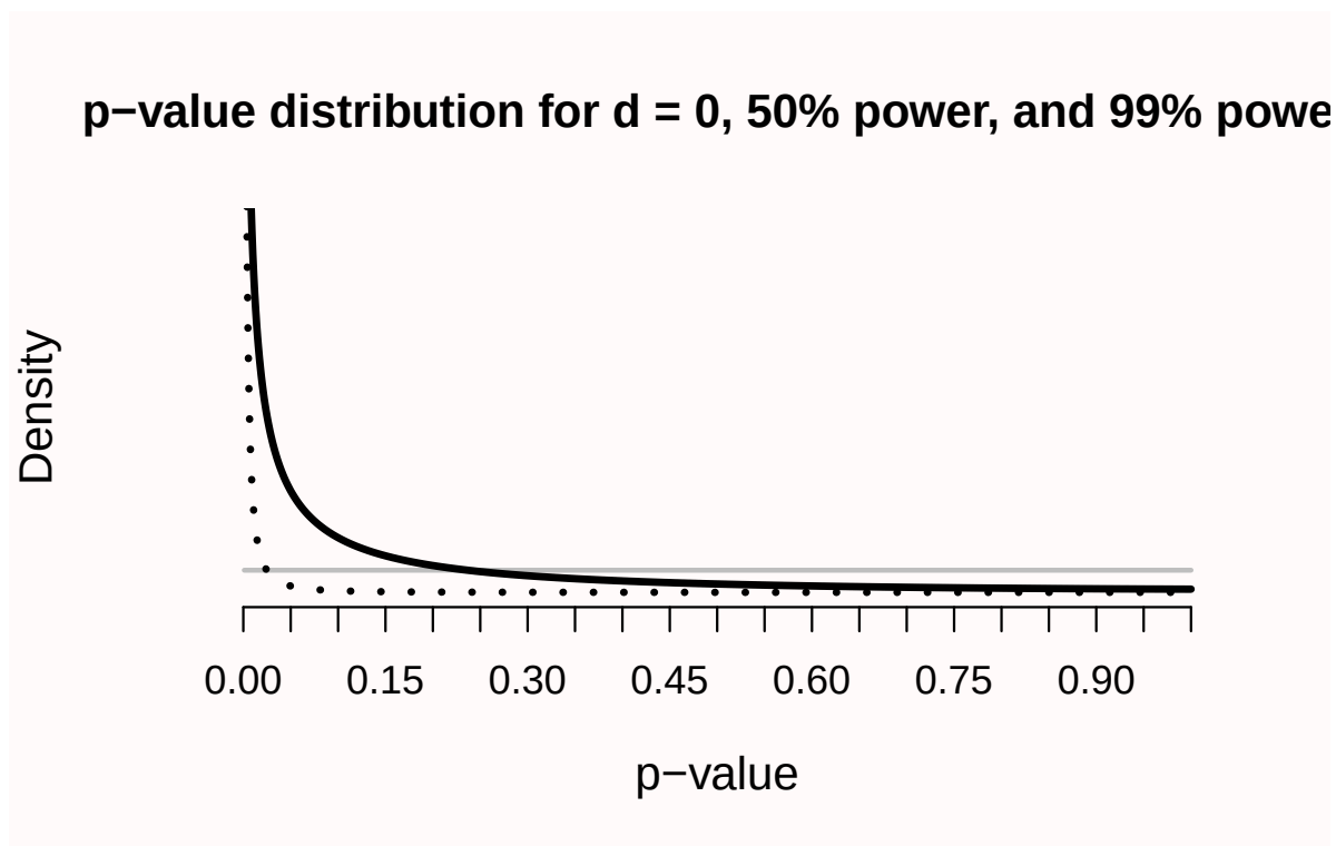
Figure 1.2: P -value distribution for 0 (grey horizontal line, 50 percent power (black solid curve), and 99 percent power (black dotted curve, where p -values just below 0.05 are more likely when H_0 is true than when H_1 is true).
