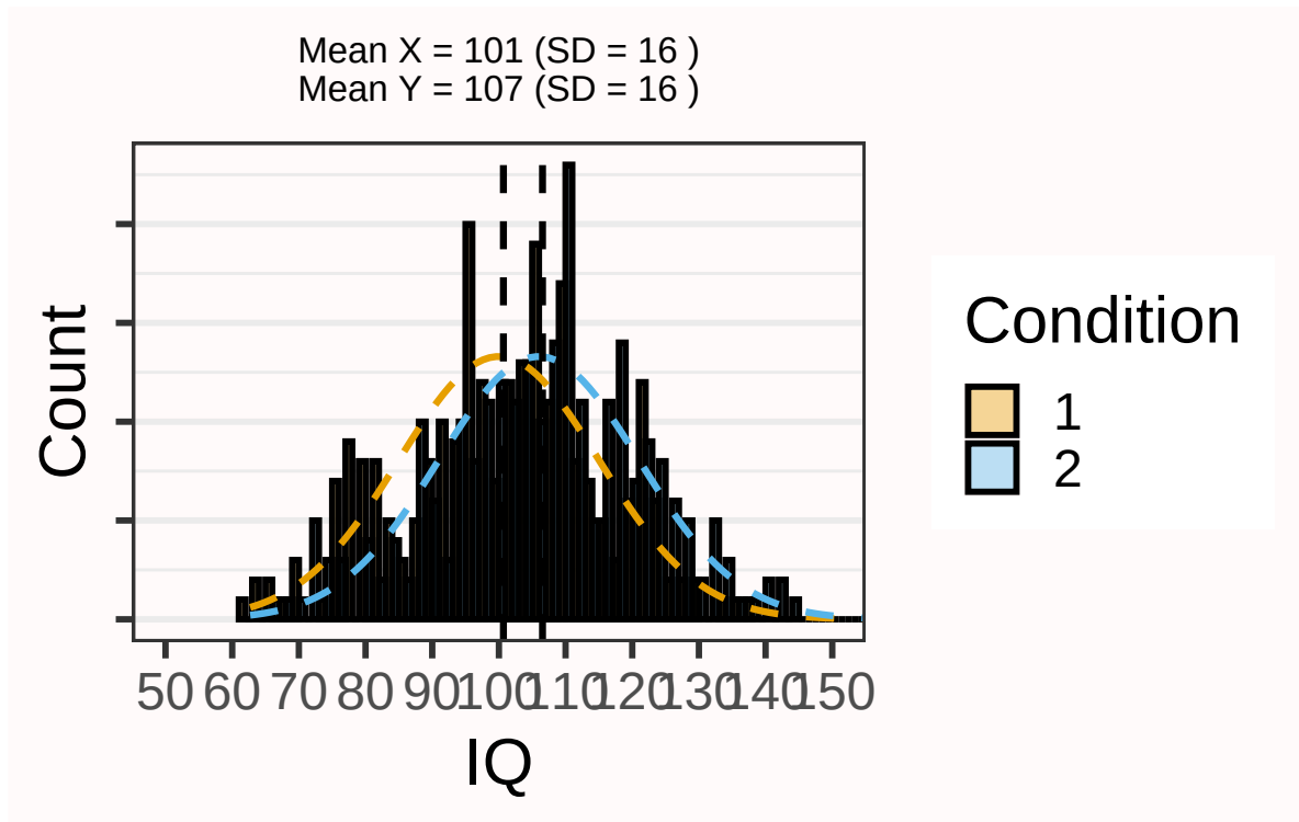
Figure 11.2: Simulated sample of 250 independent observations.
