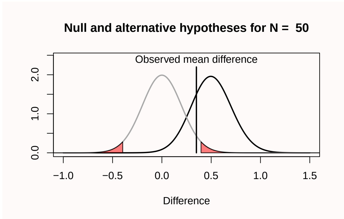
Figure 1.7: Distribution of observed Cohen's d effect sizes when collecting 50 observations per group in an independent t -test for d = 0 and d = 0.5 when observing d = 0.35 .
