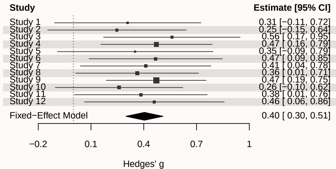
Figure 11.11: Forest plot for 12 simulated studies.
