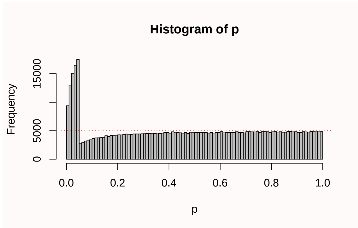
Figure 2.8: Simulation of 500000 studies performing 5 interim analyses at an alpha level of 5%.
