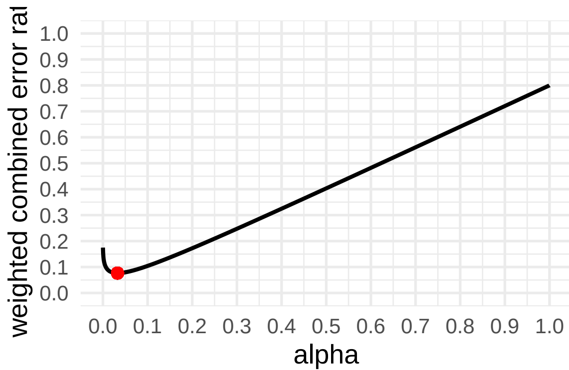
Figure 2.9: Weighted combined error rate, minimized at \alpha = 0.037 .
