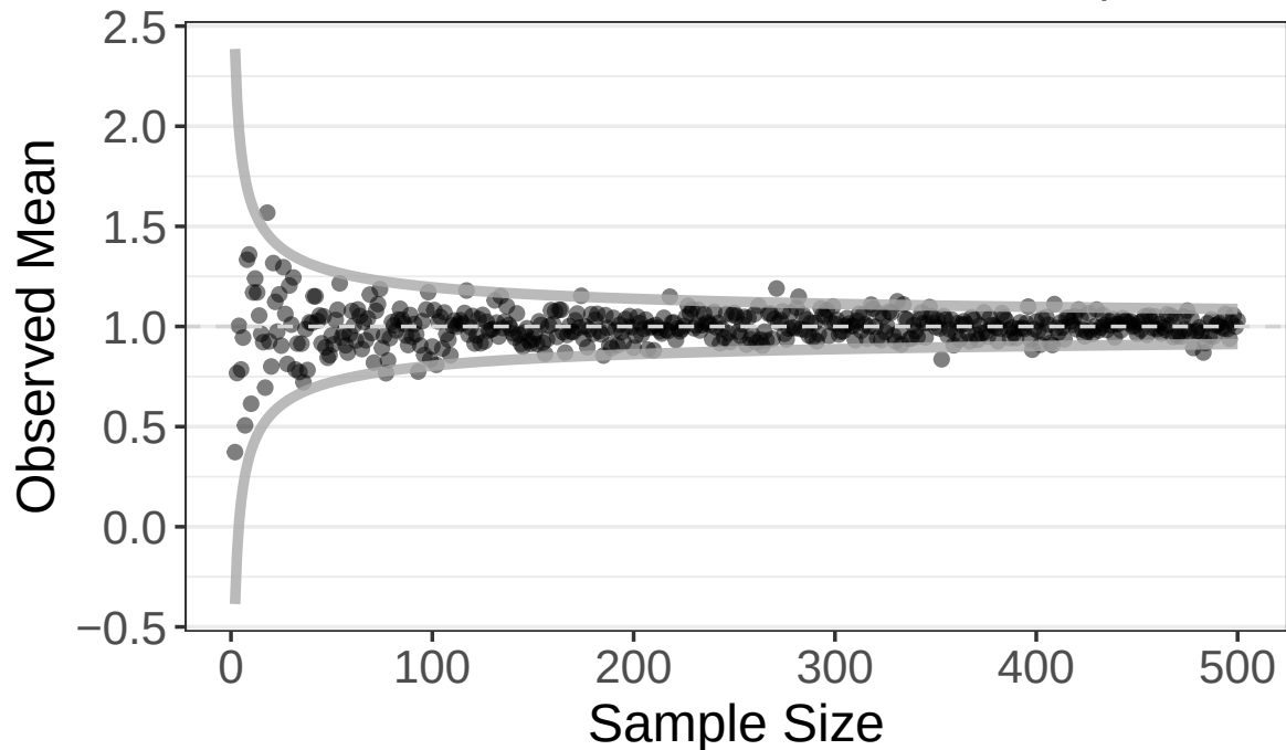
Figure 7.2: The observed mean for 500 samples drawn from a population with a true mean of 1 as the sample size increases to 500 observations. Grey lines indicate the upper and lower 95% confidence interval around the mean.
