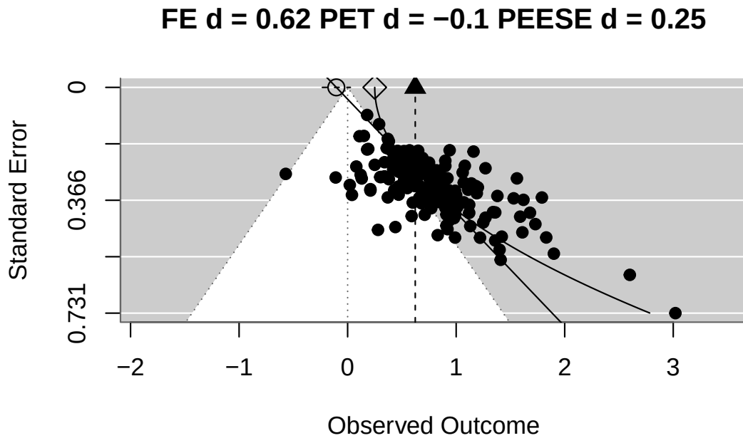
Figure 12.7: Funnel plot from Carter and McCullough (2014) visualizing bias in 198 published tests of the ego-depletion effect, including PET-PEESE bias-corrected effect size estimates.
