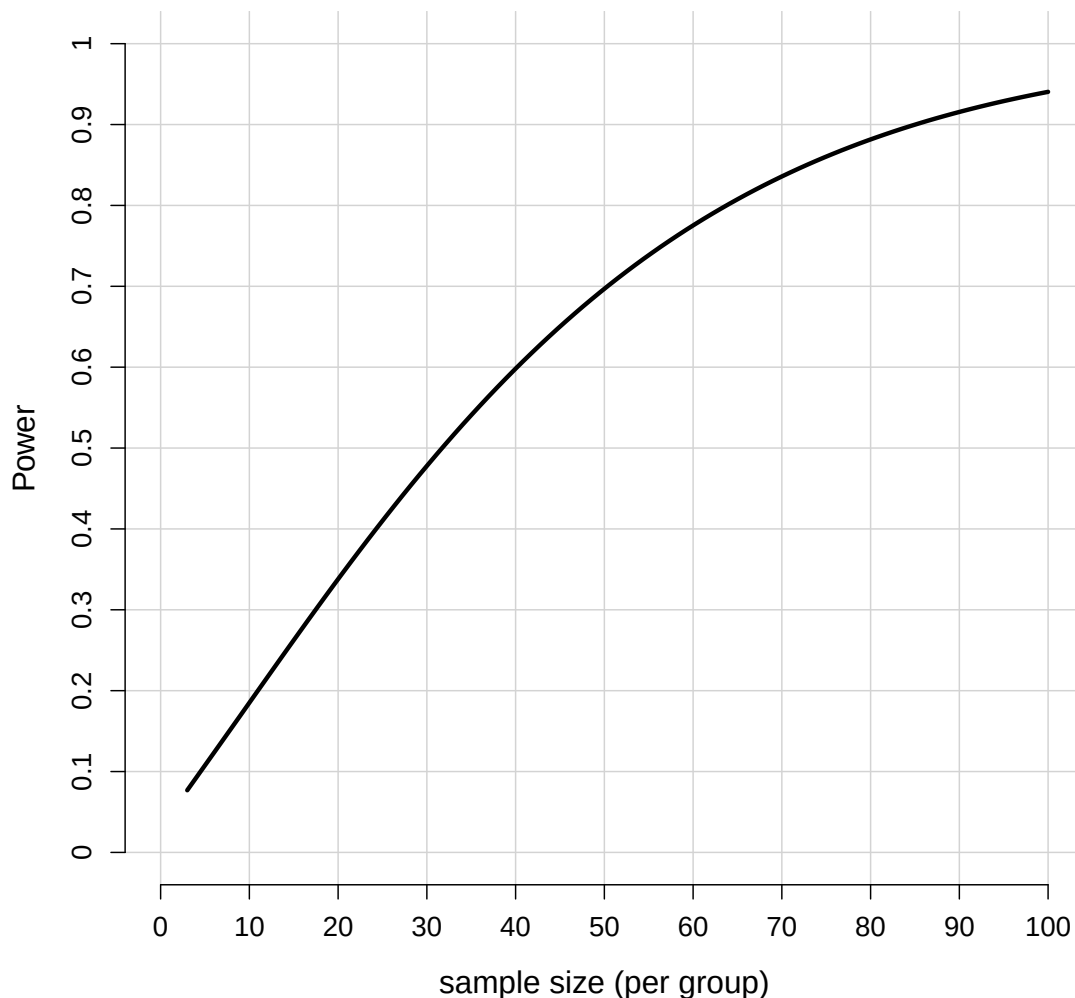
Figure 8.1: Power curve for an independent t test with an effect of d = 0.5 and \alpha = 0.05 as a function of the sample size.
