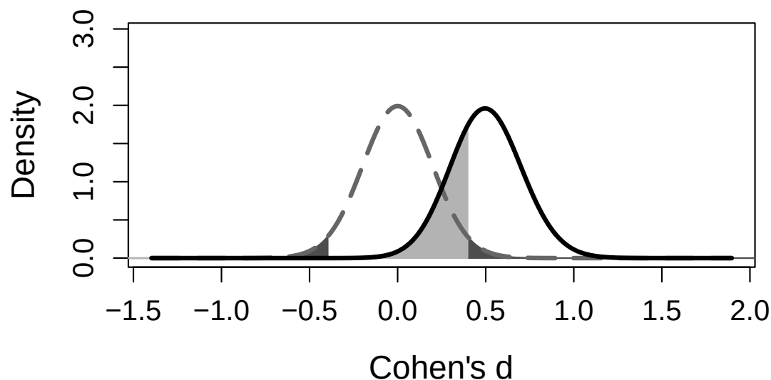
Figure 8.2: Null ( d = 0 , grey dashed line) and alternative ( d = 0.5 , solid black line) hypothesis, with \alpha = 0.05 and n = 80 per group.
