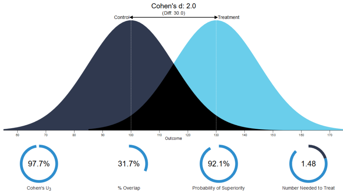
Figure 6.4: A vizualization of 2 groups representing d = 2 .
