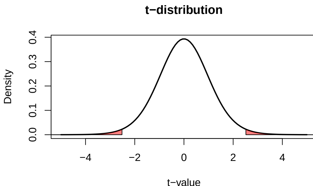
Figure 1.1: A t -distribution with 18 degrees of freedom.
