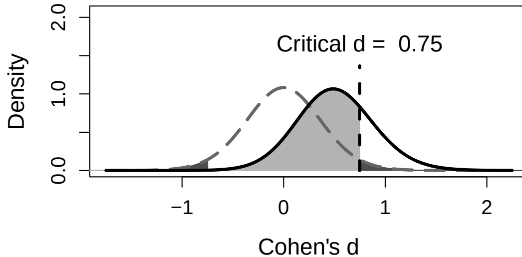
Figure 8.4: Critical effect size for an independent t test with n = 15 per group and \alpha = 0.05 .
