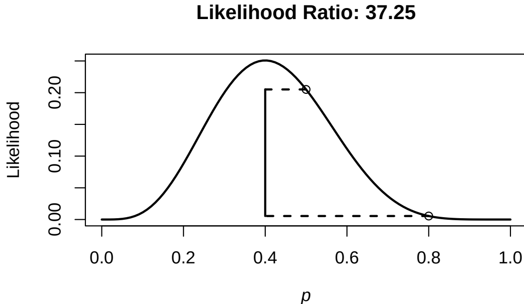
Figure 3.6: Computing a likelihood ratio for p = 0.5 relative to p = 0.8 when observing p = 0.4 .
