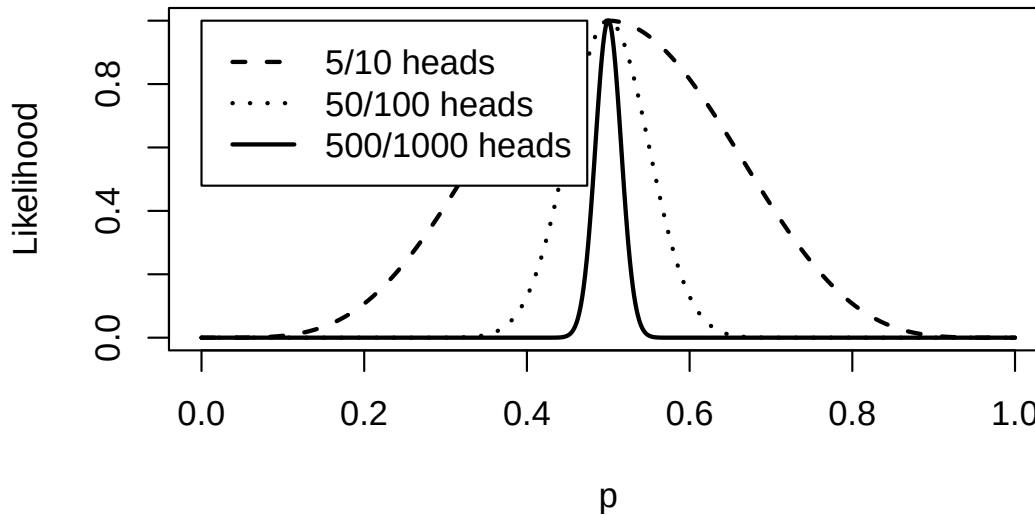
Figure 3.4: Likelihood function for 5/10, 50/100 and 500/1000 heads in coin flips.
