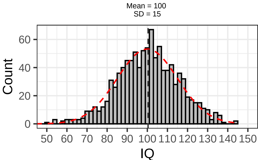
Figure 11.1: 1000 random datapoints with mean = 100 and sd = 15 in the population.
