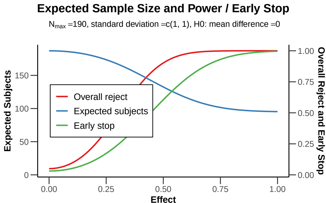
Figure 10.6: Power curve for a sequential design with 2 looks.
