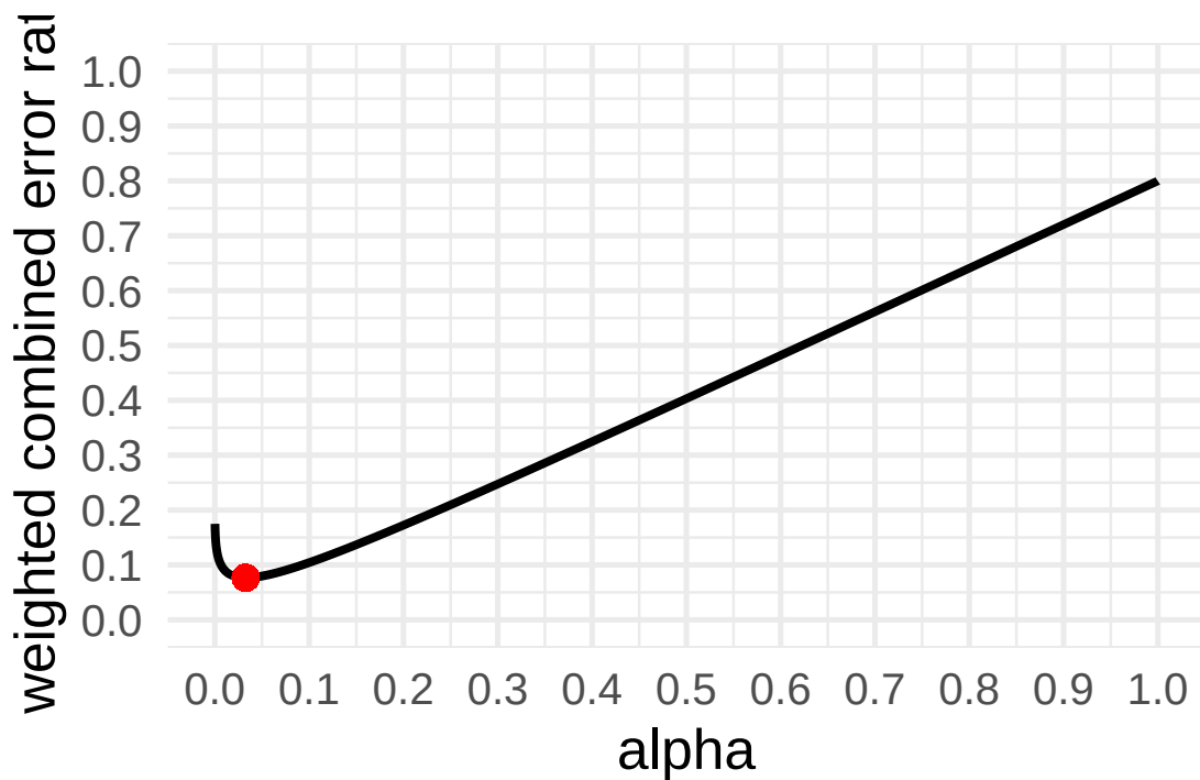
Figure 2.8: Weighted combined error rate, minimized at \alpha = 0.033 .
