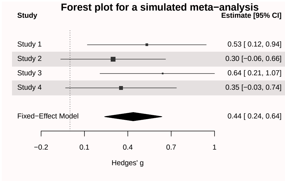
Figure 7.2: Meta-analysis of 4 studies.
