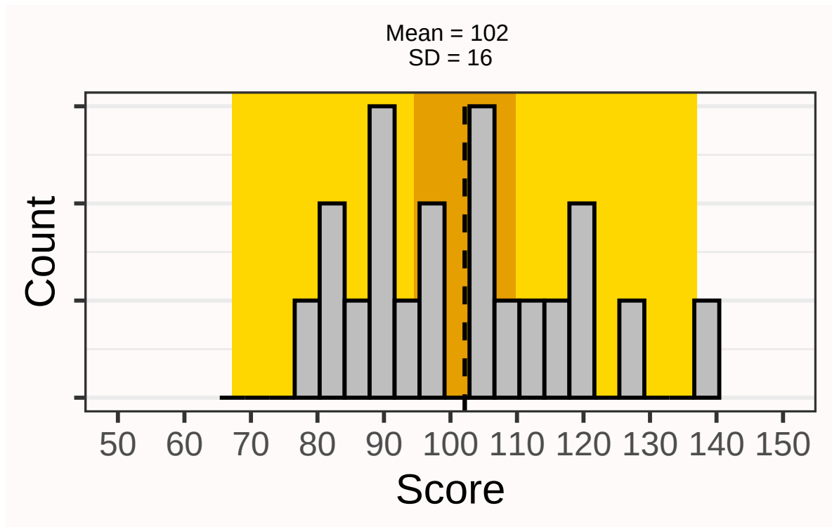
Figure 7.3: A comparison of a 95% confidence interval (orange) and 95% prediction interval (yellow).
