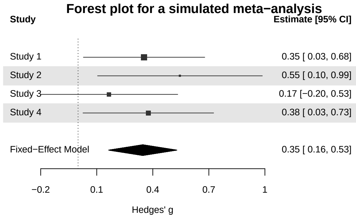
Figure 7.8: Meta-analysis of 4 studies.
