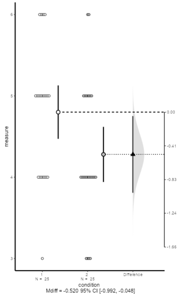
Figure 7.5: Output from ESCI module in jamovi.
