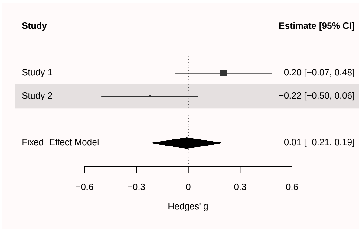
Figure 7.4: Meta-analysis of two simulated studies from the same population.
