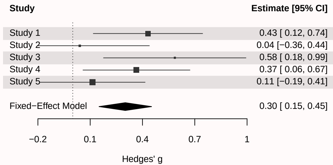
Figure 11.9: Simulated studies under a fixed effect model.
