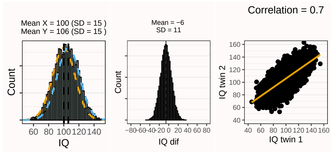
Figure 8.12: Distributions of two independent groups with means 100 and 106 and a standard deviation of 15, distribution of the differences, and correlation of 0.7.
