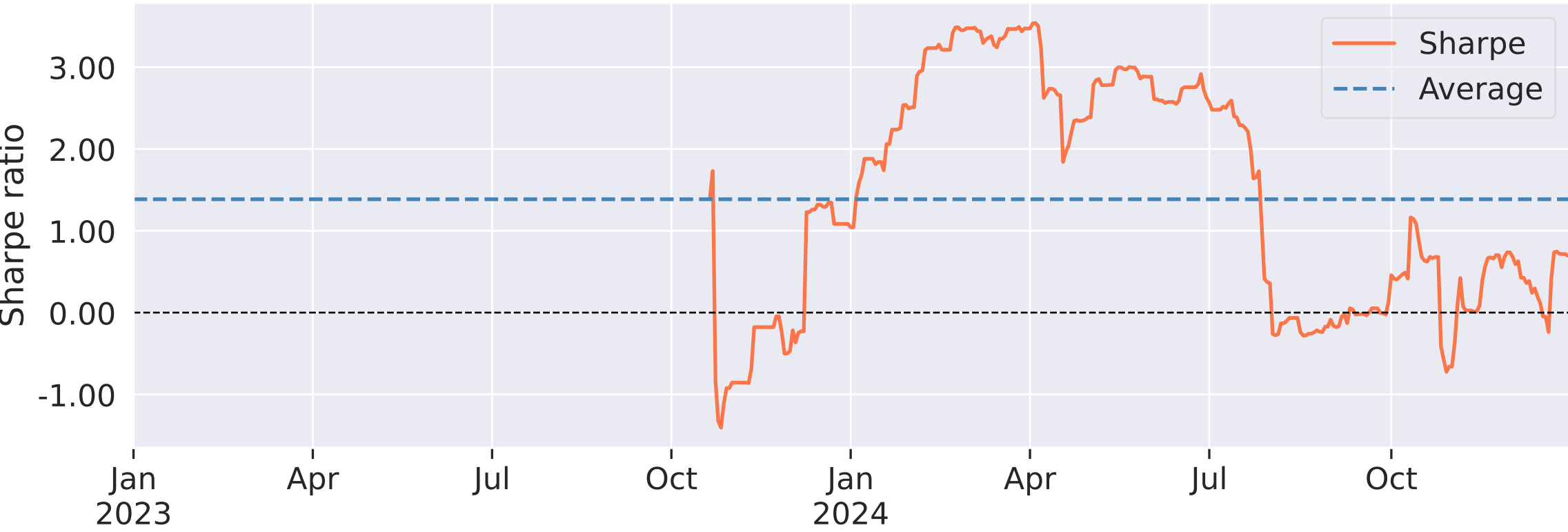
Rolling Sharpe ratio (6-month)
