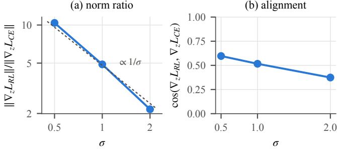
Fig. 5. E3 at fixed \sigma : (a) the RL/CE gradient-norm ratio follows 1/\sigma ; (b) alignment with the CE gradient falls as \sigma grows.
