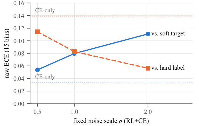
Fig. 3. As fixed \sigma grows, target-referenced ECE rises while hard-label ECE falls: the same models ranked in opposite order. Dotted lines show CE-only.
