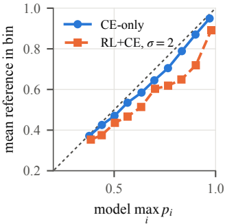
(a) vs. soft target t[\arg \max p]
