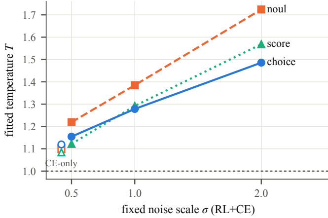
Fig. 4. Fitted temperature per question type versus fixed \sigma (RL+CE); hollow markers show CE-only. T > 1 means the raw outputs are sharper than the targets.
