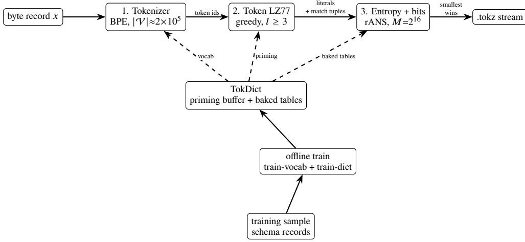
Figure 1: The TokPress pipeline: tokenize → token-level LZ77 → entropy-coded bitstream, with the trained TokDict supplying the vocabulary, an LZ priming buffer (so matches can reach into other records), and baked order-0/order-1 tables.
