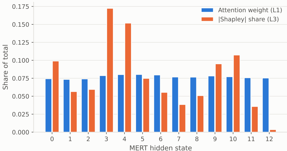
What the model weights vs what moved the decision
