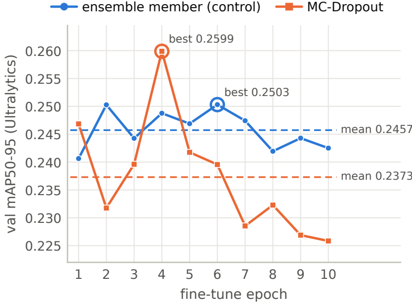
Figure 6: The best-epoch convention rewards the noisiest run. Validation mAP50-95 (Ultralytics, training-time logs) per fine-tune epoch for two VIS runs sharing machine, seed and recipe: an ensemble member (control) and MC-Dropout. Rings mark the epoch best.pt keeps; dashed lines are the 10-epoch means. MC-Dropout reads +0.0096 better by best epoch and -0.0084 worse by epoch mean. Sources: runs/ensemble/ens_vis_seed0_ft_control/results.csv , runs/mc_dropout/mc_vis_seed0_ft_refit/results.csv ; decision record docs/D31-checkpoint-selection-2026-09-01.md.
