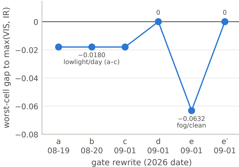
Figure 7: Worst-cell gap of gated fusion to max(VIS, IR) across the six gate rewrites (Table 11), pre-restore checkpoints (yolo26s for a–d, yolo26m from e), development paired frames, ship AP (local AP). Each rewrite was forced by the failure of the one before it; stages a–c share their worst cell, lowlight/day. Stage e is the detector swap to yolo26m, which turned the fog veto into a -0.0632 regression without any change to the images.
