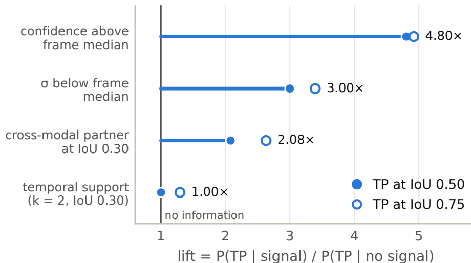
Figure 5: Which per-box signals predict a true positive. Lift = P(\text{TP} \mid \text{signal fires}) / P(\text{TP} \mid \text{it does not}) , VIS boxes on the clean day frames of the paired set, full-scale pre-restore yolo26m caches. A signal at lift 1.0 carries no information, and no weight placed on it can change an AP ranking. Filled: true positive at IoU 0.50; hollow: at IoU 0.75. Temporal support is a box at \text{IoU} \geq 0.30 in one of the two preceding frames. Source: runs/eval/signal_lift_26m.md .
