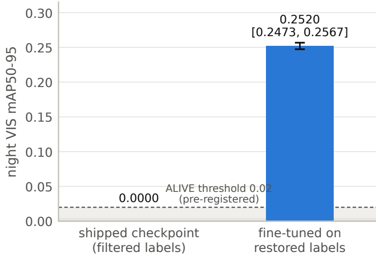
Figure 4: Night VIS mAP50-95 before and after the label restore. 2,068 pohang01 validation frames, 16,179 ground-truth boxes, all ship, so mAP50-95 is ship AP. The interval is the paired bootstrap interval (1,000 resamples) on the difference, which equals the new arm because the old arm scores 0.0000. The dashed line is the pre-registered ALIVE threshold (0.02); the shaded strips below it are the WEAK (0.005–0.02) and DEAD (< 0.005) bands. Source: runs/eval/night_restore_verdict.md , bands fixed in docs/prereg-night-label-restore.md .
