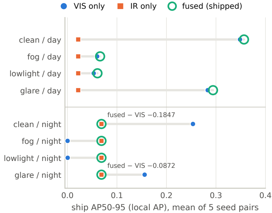
Figure 3: The shipped rule on the five Phase 3 systems (Table 2), ship AP (local AP), seed mean. By day the fused output sits just above VIS alone on every cell. At night VIS is vetoed on every frame, so the fused output equals IR alone: right where VIS fails (fog, low light), wrong where it still works (clean, glare). Sources: docs/eval/p3_night_check_2026-09-27.json , docs/eval/p3_corrupt_cells_2026-09-27.json .
