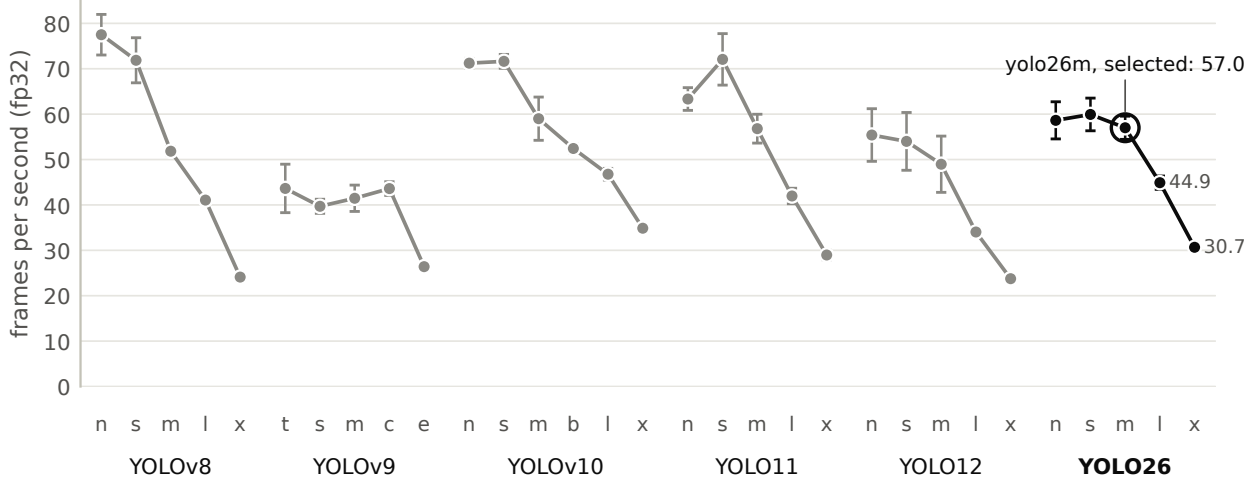
Figure 6: Batch-1 throughput of the 31 Phase 1 variants, one size ladder per family, fp32, seed mean \pm sd. One detector’s predict() per frame at 640 \times 640 , 500 timed frames after 50 warm-up, GPU clock pinned at 1500 MHz on the laptop of Appendix M (RTX 4080 Laptop); three seeds per variant (two for yolo12x). The sd is measurement precision, not architectural variation: the seeds of a variant share its architecture. The fusion runs one detector per modality, so two-stream throughput is half these values (Table 10), before the \sigma head, image statistics and decision layer, which are not timed (§9). yolo26m, ringed, is the selected backbone. Source: phase1_benchmark/fps.csv .
