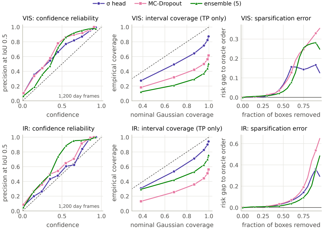
Figure 2: Per-stream calibration of the three uncertainty arms, day slice (1,200 of the 2,232 paired validation frames), no fusion; the primary basis of Table 1. Left: precision at IoU 0.5 against confidence in D-ECE’s ten bins (bins with at least 20 boxes). Middle: empirical against nominal Gaussian coverage of |\text{error}| \leq k\sigma for k = 0.5\text{--}3 , true positives only; for MC-Dropout and the ensemble \sigma is member disagreement (§6.2). Right: risk ( 1 - \text{IoU} , a false positive counting 1) of the retained boxes minus the oracle ordering’s, as the most uncertain boxes are removed; its mean over the grid is AUSE. Dashed lines are perfect calibration. Recomputed from Table 1’s caches with the same metric code: D-ECE and interval-ECE reproduce Table 1 exactly, AUSE and AURC to within the spread across tie orders (see Table 1’s note). Source: docs/eval/uq_day_night_slice_u2_nanpolicy_2026-09-09.md.
