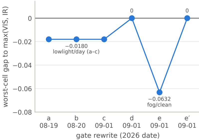
Figure 9: Worst-cell gap of gated fusion to max(VIS, IR) across the six gate rewrites (Table 11), pre-restore checkpoints (yolo26s for a–d, yolo26m from e), development paired frames, ship AP (local AP). Each rewrite was forced by the failure of the one before it; stages a–c share their worst cell, lowlight/day. Stage e is the detector swap to yolo26m, which turned the fog veto into a -0.0632 regression without any change to the images.
