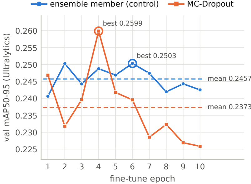
Figure 8: The best-epoch convention rewards the noisiest run. Validation mAP50-95 (Ultralytics, training-time logs) per fine-tune epoch for two VIS runs sharing machine, seed and recipe: an ensemble member (control) and MC-Dropout. Rings mark the epoch best.pt keeps; dashed lines are the 10-epoch means. MC-Dropout reads +0.0096 better by best epoch and −0.0084 worse by epoch mean. Sources: runs/ensemble/ens_vis_seed0_ft_control/results.csv , runs/mc_dropout/mc_vis_seed0_ft_refit/results.csv ; decision record docs/D31-checkpoint-selection-2026-09-01.md .
