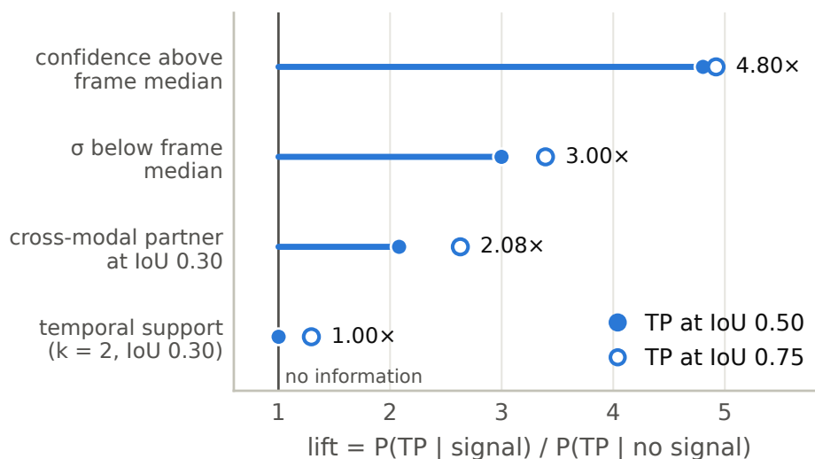
Figure 7: Which per-box signals predict a true positive. Lift = P(\text{TP} \mid \text{signal fires}) / P(\text{TP} \mid \text{it does not}) , VIS boxes on the clean day frames of the paired set, full-scale pre-restore yolo26m caches. A signal at lift 1.0 carries no information, and no weight placed on it can change an AP ranking. Filled: true positive at IoU 0.50; hollow: at IoU 0.75. Temporal support is a box at \text{IoU} \geq 0.30 in one of the two preceding frames. Source: runs/eval/signal_lift_26m.md .
