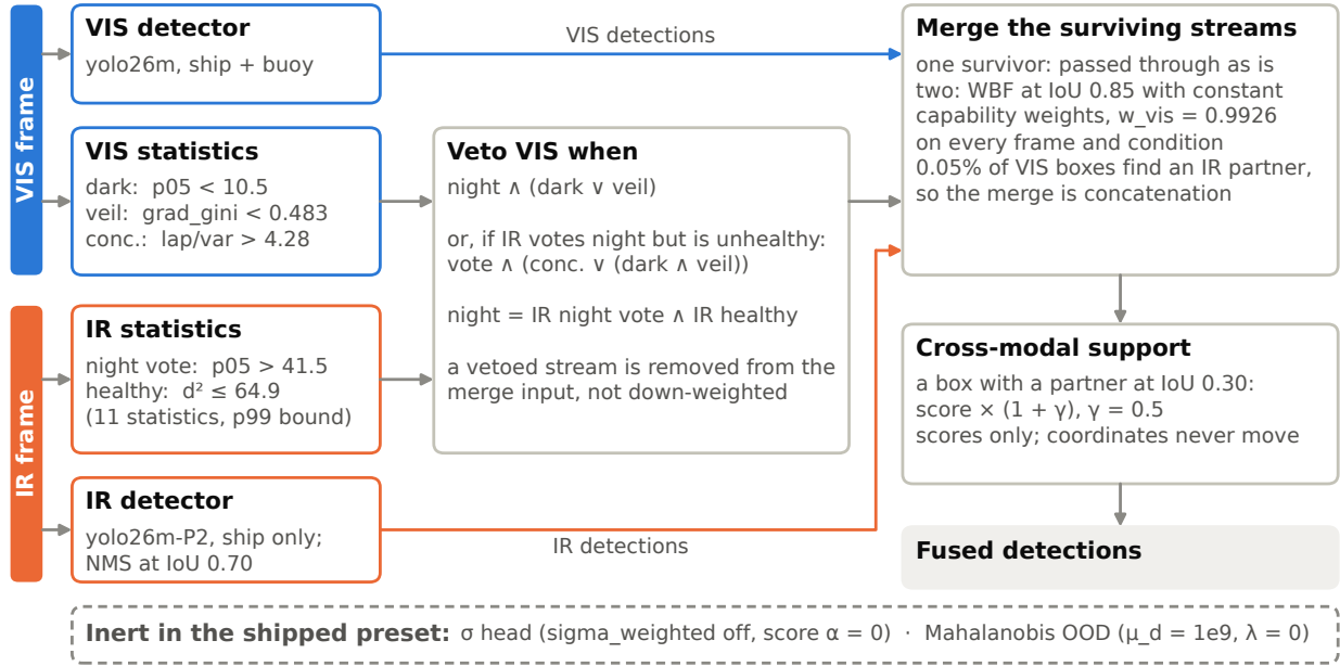
Figure 1: The shipped decision layer (preset crossmodal126m). Frame statistics from both streams drive a hard veto on VIS; the surviving streams are merged by WBF with constant capability weights, so w_{\text{vis}} = 0.9926 on all 2,232 paired frames and all four conditions, and at IoU 0.85 the merge is concatenation. A cross-modal partner at IoU 0.30 raises a box’s score and never moves it. Thresholds are the frozen constants the code loads ( runs/eval/structure_constants.json , runs/eval/brightness_constants.json ); the night threshold and the IR health model are fitted in-sample (§9). The \sigma head and the Mahalanobis score are computed but inert.
