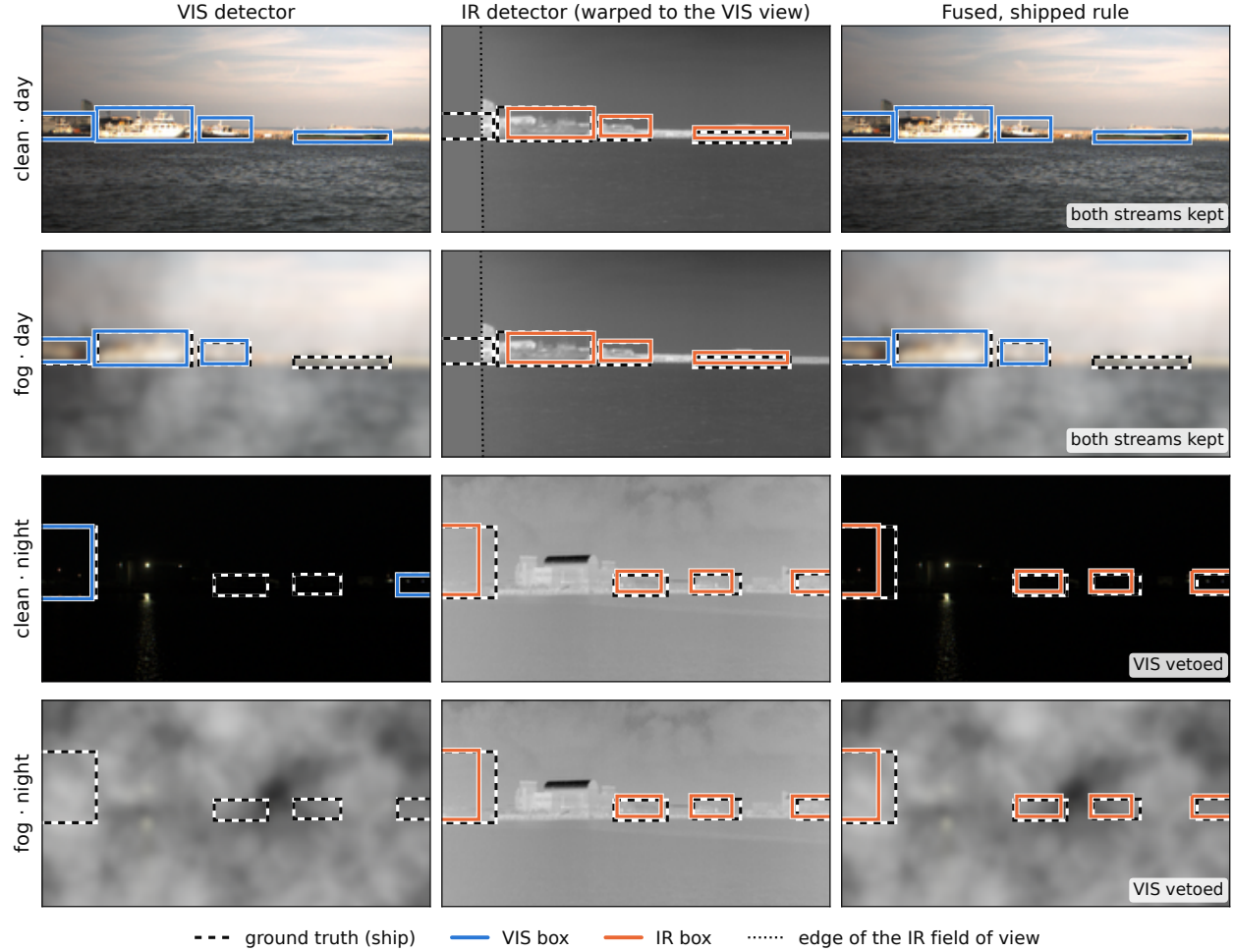
Figure 5: The shipped rule on one day frame and one night frame, clean and fogged. Phase 3 system seed 0 (VIS seed 0 with IR seed 0), preset crossmodal26m , development paired frames. Fog is VIS draw 941 at severity 2, regenerated with the cache builder’s own call; IR is clean in every row, as in every Table 2 cell. The two frames were drawn at random (seed 0) among paired frames with at least three ground-truth ships inside the IR field of view, of median height at least 15 px; no detection entered the choice. Each panel is a 320 \times 170 crop of the 640 \times 640 canvas, and IR frames are warped into the VIS view by the per-frame homography the fusion uses, so the three columns share one geometry. Ship class only, boxes at confidence \geq 0.25 , fused boxes coloured by the stream they came from. By day the veto does not fire and both streams enter the merge, but IR boxes enter with their scores scaled by the IR capability weight (§4.2), far below the display threshold, so only VIS boxes are drawn; the far ship that fogged VIS misses has an IR box, which reaches the fused list only at that reduced score. At night the IR vote drops VIS on both frames. On the fogged frame VIS finds nothing, and dropping it is right, as in the fog/night cell. On the clean frame VIS has found ships, and its boxes are discarded anyway: the rule reads darkness, not what the visible detector found. IR boxes cover more of these ships but overlap the ground truth less (best IoU 0.53–0.63, against 0.69–0.92 for VIS), and AP50-95 averages over IoU thresholds up to 0.95. One frame shows the mechanism, not the cost; over the clean night cell the cost is the 0.1847 above. Source: scripts/fig_detections.py ; frames, crops, flags and IoUs in docs/figures/fig_detections.json .
