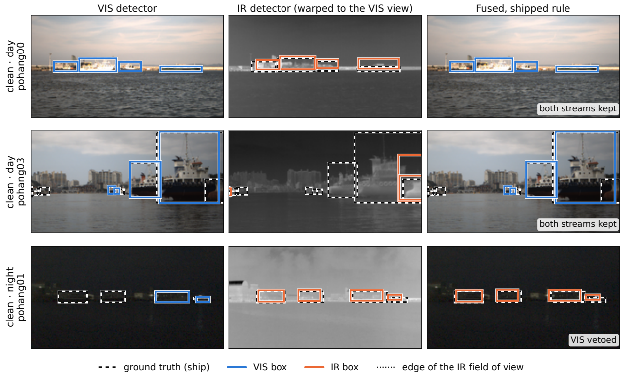
Figure 11: Three further scenes, clean. Same system, selection and display as Figure 5: a quay in pohang00 and a tug beside a large ship in pohang03 by day, a row of moored ships in pohang01 by night. By day the fused output shows the VIS boxes. At night VIS has found two of the ships (best IoU 0.73 and 0.95) and is vetoed; IR finds more of the row, three of its boxes at IoU 0.66–0.77 to the ground truth. Source as Figure 5.
