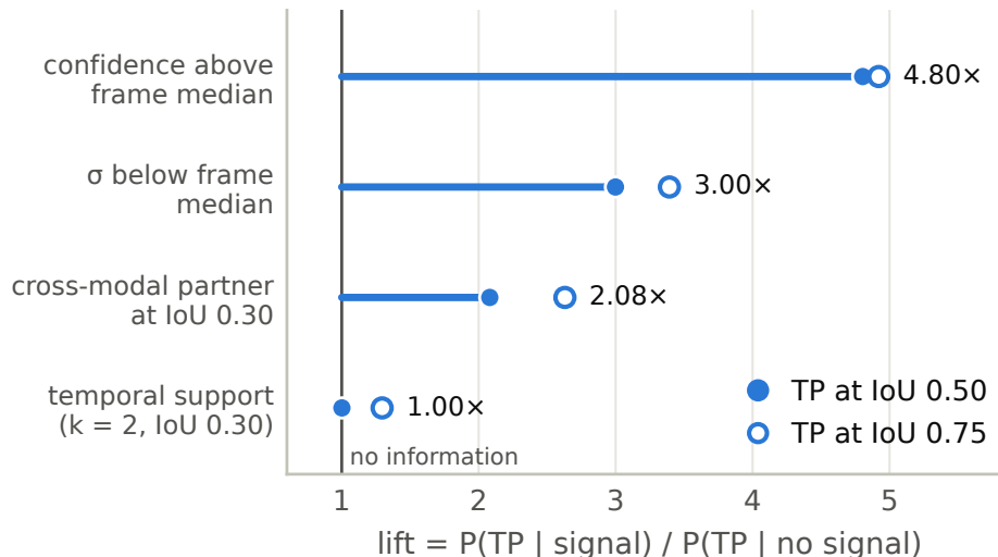
Figure 7: Which per-box signals predict a true positive. Lift = P(\text{TP} \mid \text{signal fires}) / P(\text{TP} \mid \text{it does not}) , VIS boxes on the clean day frames of the paired set, full-scale pre-restore yolo26m caches. A signal at lift 1.0 carries no information, and no weight placed on it can change an AP ranking. Filled: true positive at IoU 0.50; hollow: at IoU 0.75. Temporal support is a box at \text{IoU} \geq 0.30 in one of the two preceding frames. Source: runs/eval/signal_lift_26m.md .
