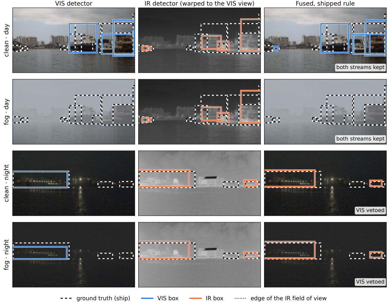
Figure 5: The shipped rule on one day frame and one night frame, clean and fogged. Phase 3 system seed 0 (VIS seed 0 with IR seed 0), preset crossmodal26m , development paired frames (pohang03 by day, pohang01 by night). Fog is VIS draw 941 at severity 2 under corruption v2 (§5.1), regenerated with the cache builder’s own call; IR is clean in every row, as in every Table 2 cell. Frames were chosen for legibility by visual review of renders that showed ground truth only, never a detection ( scripts/fig_detections.py -candidates ), and the crops were set in the same review. Each panel is a 320 \times 170 crop of the 640 \times 640 canvas; IR is warped into the VIS view by the per-frame homography the fusion uses; night VIS is brightened for display only (gamma 0.45), and the detector saw the stored frame. Ship class only, boxes at confidence \geq 0.25 , fused boxes coloured by the stream they came from. By day the veto does not fire and both streams enter the merge, but IR boxes enter with their scores scaled by the IR capability weight (§4.2), below 0.02 here, so the fused output shows VIS boxes. Two VIS boxes below the display threshold (0.20 and 0.18) appear in it because an IR box overlapping each at \text{IoU} \geq 0.30 raised its score through the support term (§4.2). Under fog VIS returns no ship box at the display threshold and the fused output shows none either, while the clean IR stream still finds the berthed ships; its boxes enter the merge scaled below the display threshold. At night the IR vote drops VIS on both frames. On the clean frame VIS has found the ferry (best IoU 0.94), and its boxes are discarded anyway; the IR boxes that replace them fit less tightly (0.75 and 0.53), and AP50-95 averages over IoU thresholds up to 0.95. On the fogged frame VIS still finds the ferry (best IoU 0.71) and is dropped as well. One frame shows the mechanism, not the cost; over the clean night cell the cost is the 0.1847 above. Source: scripts/fig_detections.py ; frames, crops, flags and IoUs in docs/figures/fig_detections.json .
