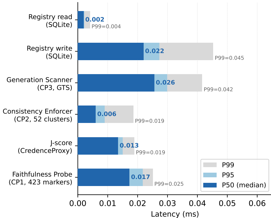
Figure 5. Per-component latency (P50 / P95 / P99, n = 500-1000 each) Total system overhead < 0.1 ms per turn at P50.
