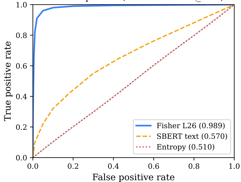
ROC comparison (PARAM vs CTX\_DEP)
