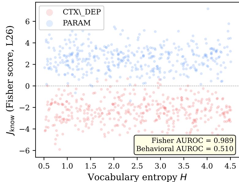
Structural independence: r = +0.004 ( n = 800 )
